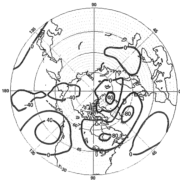
Fig. 6d. Geopotential height difference (meters) at 500 mb between averages of two anomaly runs and six control runs averaged for days 15-45.
