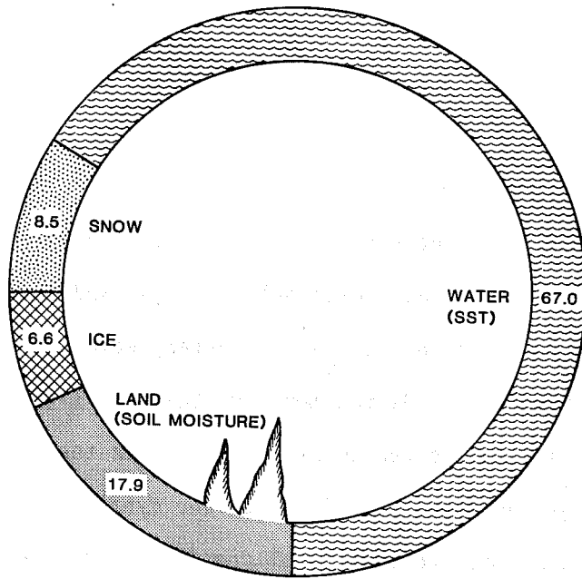
Fig. 1a. Schematic representation of the atmosphere's lower boundary. Numbers denote the percentage of earth surface area covered by different boundary forcings during January.
