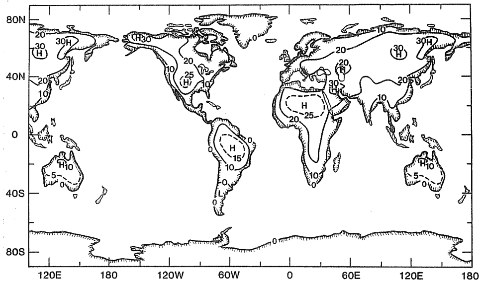
Fig. 7d. Ground temperatures (°C) difference (dry soil-wet soil) between two model simulations for the month of July.
