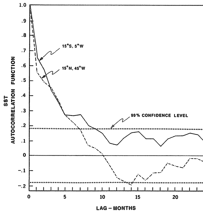
Fig. 4d. Lag correlation function for monthly mean SST anomaly at 15^{\circ} S, 5^{\circ} W and 15^{\circ} N, 45^{\circ} W. (From Moura and Shukla, 1981)
