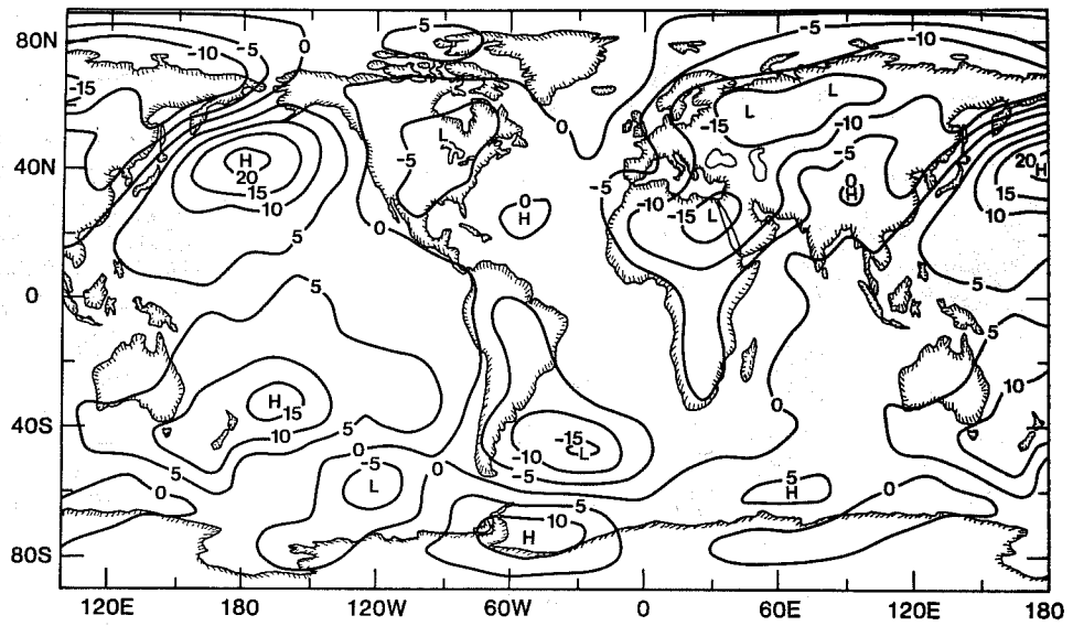
Fig. 7e. Sea level pressure (mb) difference (dry soil-wet soil) between two model simulations for the month of July.
