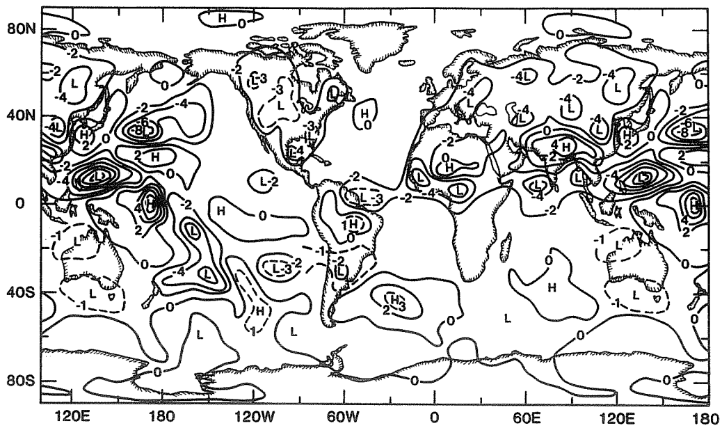
Fig. 7c. Rainfall (mm/day) difference (dry soil-wet soil) between two model simulations for the month of July.
