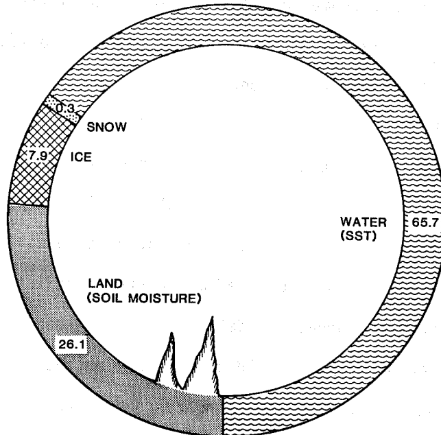
Fig. 1b. Schematic representation of the atmosphere's lower boundary. Numbers denote the percentage of earth surface area covered by different boundary forcings during July.
