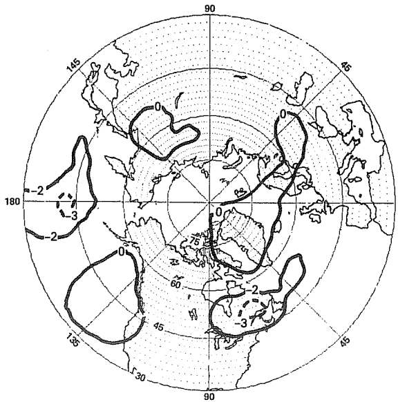
Fig. 6c. Ratio of the temperature difference at 700 mb (shown in Figure 6b) to the standard deviation among 15-45 day averages of six control runs.
