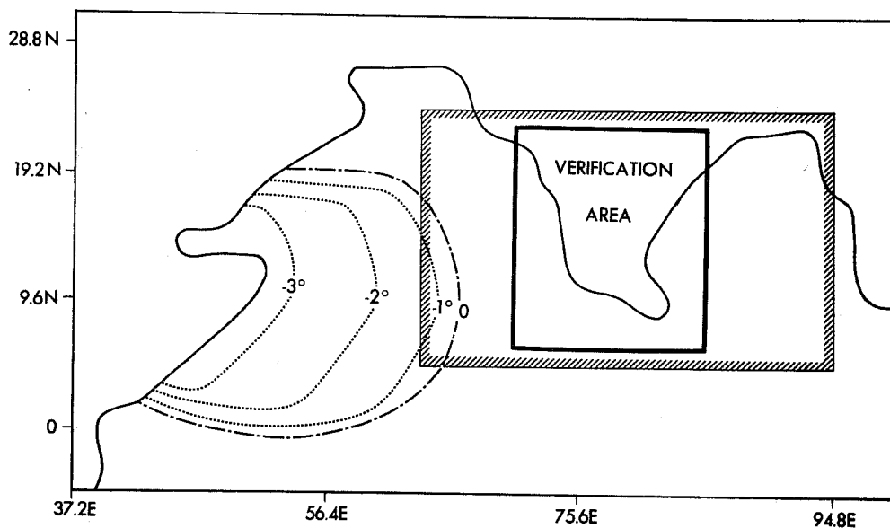
Fig. 2a. Sea surface temperature anomaly ( ^{\circ}\text{C} ) over the Arabian Sea used for the GCM experiment and the area of verification.
