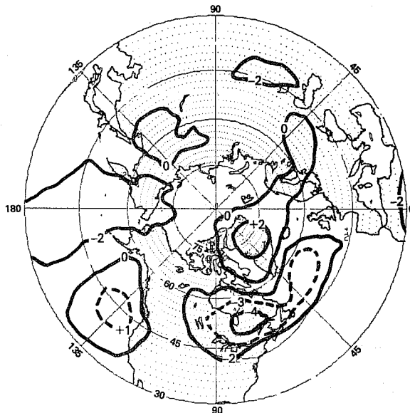
Fig. 6b. Temperature difference ( ^{\circ}\text{C} ) at 700 mb between average of two anomaly runs and six control runs averaged for days 15-45.
