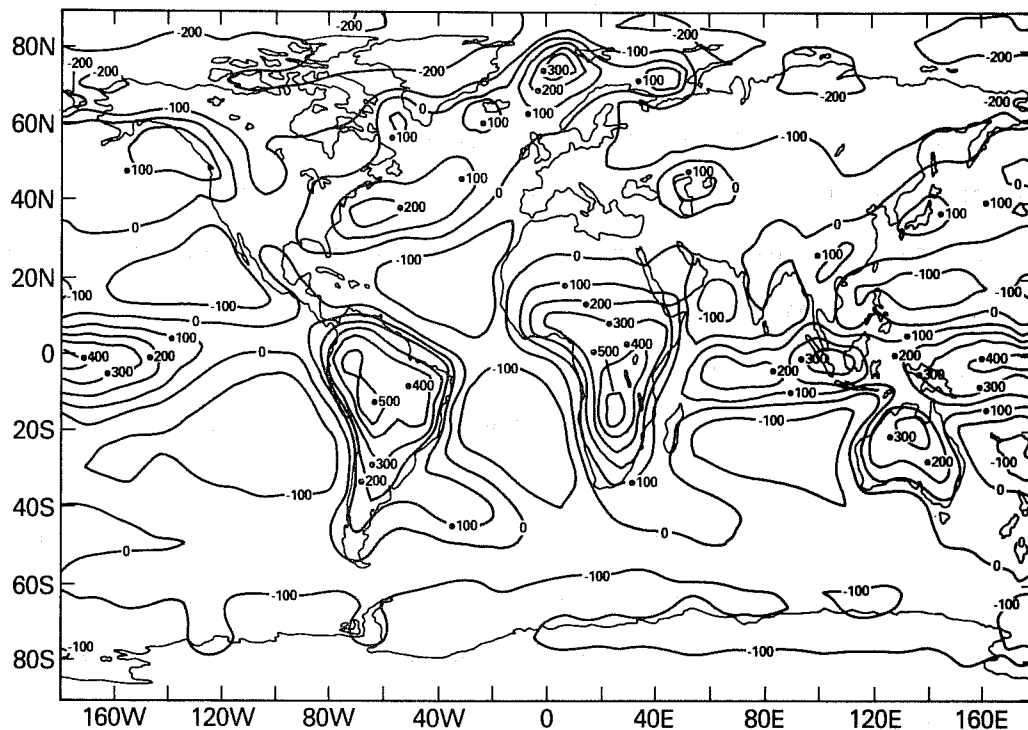
Fig. 7a. Vertically integrated net diabatic heating ( \text{cal cm}^{-2} \text{ day}^{-1} ) of the atmospheric column during winter as simulated by the GLAS climate model.
