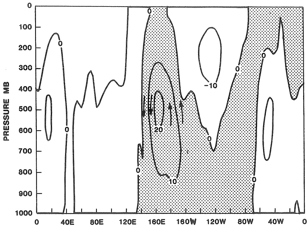
Fig. 5d. Difference (anomaly-control) of Walker cell (in units of 10^9 kg/sec) averaged between 6^{\circ}\text{N} - 6^{\circ}\text{S} and averaged for days 6-25.
