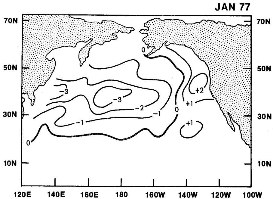
Fig. 6a. Sea surface temperature anomaly ( ^{\circ}\text{C} ) over north Pacific used for the GCM experiment. This anomaly pattern will be identical to the observed SST anomaly during January 1977 if units are changed from ( ^{\circ}\text{C} ) to ( ^{\circ}\text{F} ).
