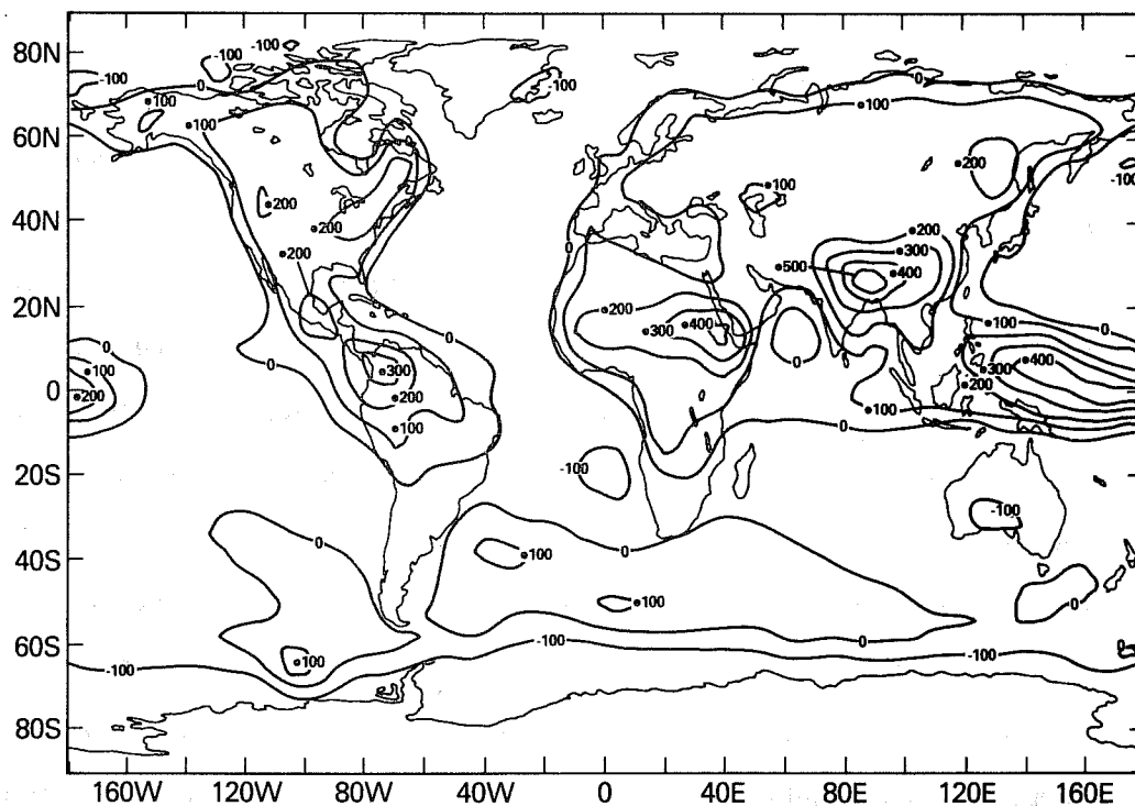
Fig. 7b. Vertically integrated net diabatic heating ( \text{cal cm}^{-2} \text{ day}^{-1} ) of the atmospheric column during summer as simulated by the GLAS climate model.
