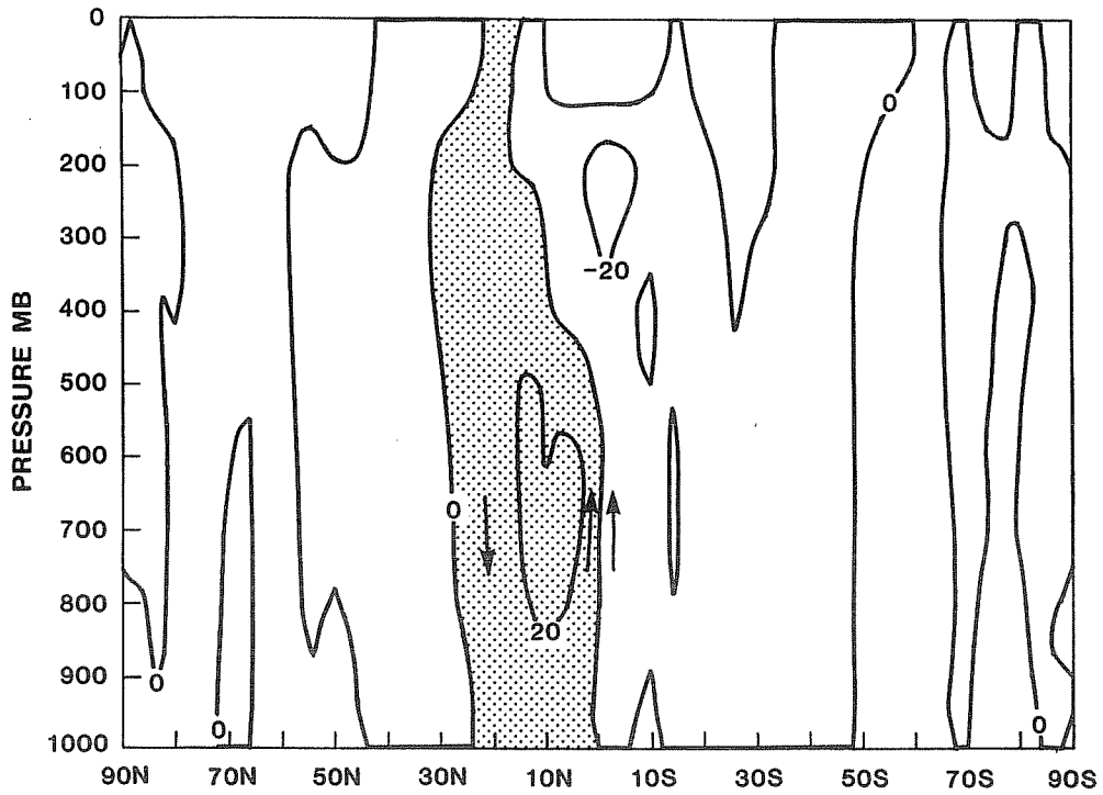
Fig. 5c. Difference (anomaly-control) of Hadley cell (in units of 10^9 kg/sec) averaged for days 6-25.
