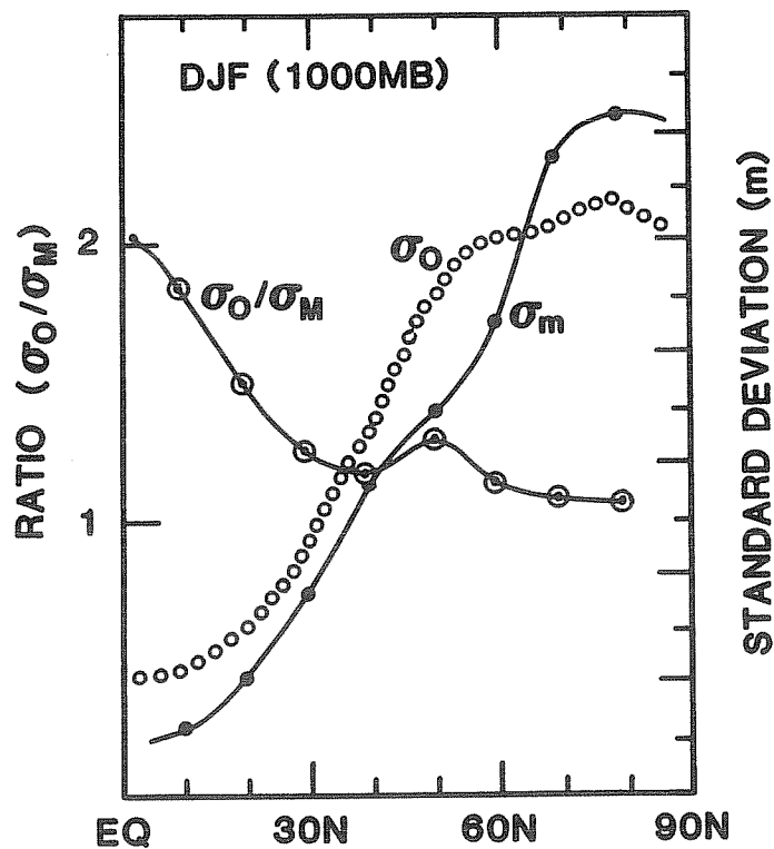
Fig. 10a. Zonal means of standard deviation of daily and monthly mean 1000 mb geopotential height (m) for the Dec.-Jan.-Feb. season. Observed distributions are from Oort and Jenne. The ratio of observed and model standard deviation is on the left hand side. (from Manabe and Hahn, 1981).
