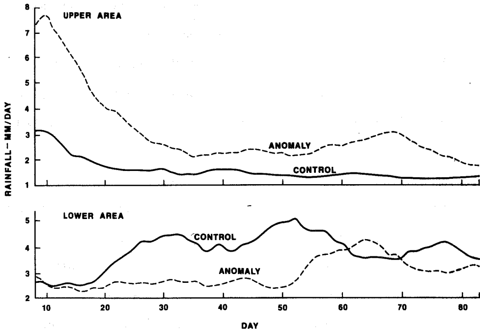
Fig. 4b. 15 day running mean of daily rainfall (mm/day) for upper (area A) and lower (area B) areas. (From Moura and Shukla, 1981).
