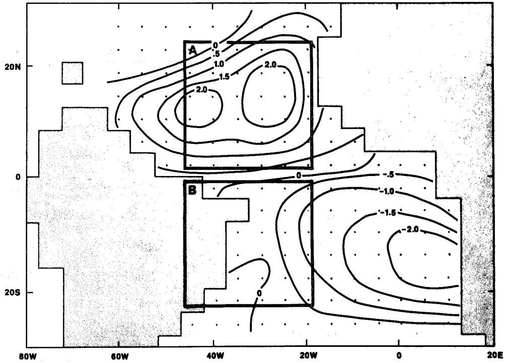
Fig. 4a. Sea surface temperature anomaly ( ^{\circ}\text{C} ) over tropical Atlantic used for the GCM experiment.
