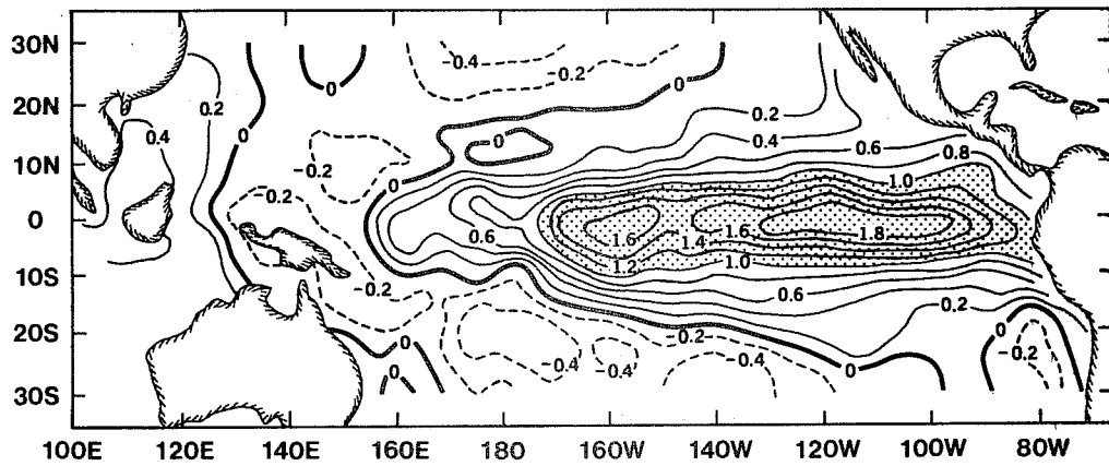
Fig. 5a. Sea surface temperature anomaly ( ^{\circ}\text{C} ) used for the GCM experiment.
