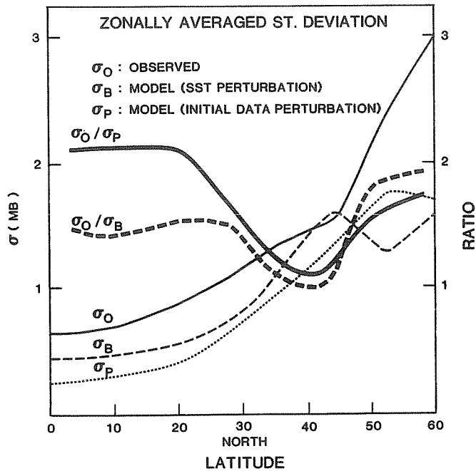
Fig. 9. Zonally averaged standard deviation among monthly mean (July) sea level pressure (mb) for 10 years of observations ( \sigma_O , thin solid line); four model runs with variable boundary conditions ( \sigma_B , thin dashed line); and four model runs with identical boundary conditions ( \sigma_P , thin dotted line). Thick solid line and thick dashed line show the ratio \sigma_O/\sigma_P and \sigma_O/\sigma_B respectively.
