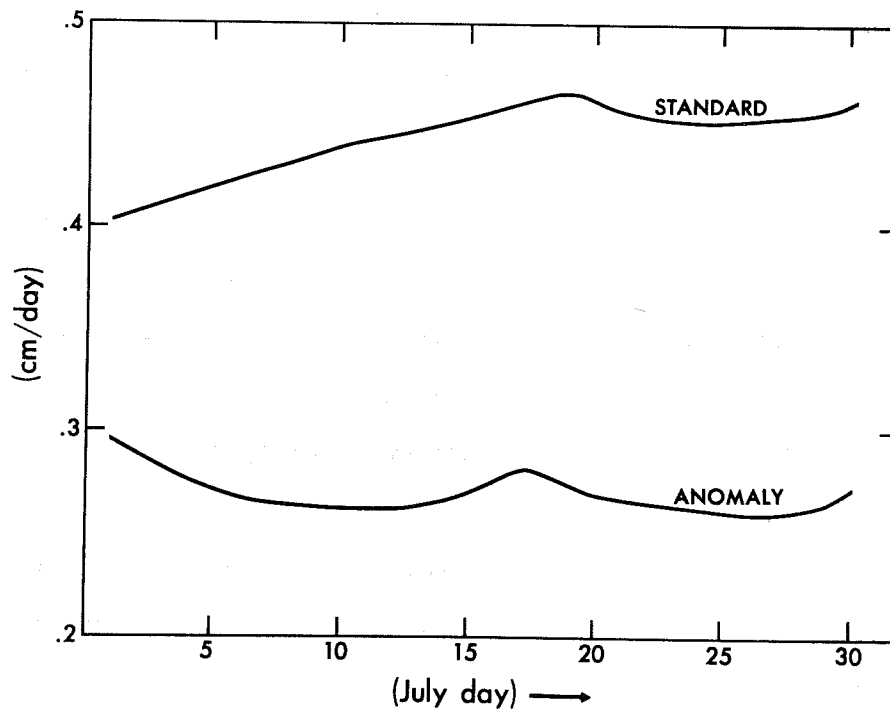
Fig. 2b. 15 day running mean of the rate of precipitation ( \text{cm day}^{-1} ) averaged over the verification area for the standard and anomaly runs.
