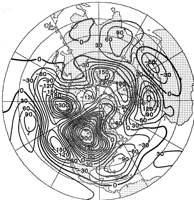
Fig. 5b. Difference (anomaly-control) of 300 mb geopotential height field averaged for days 11-25.
