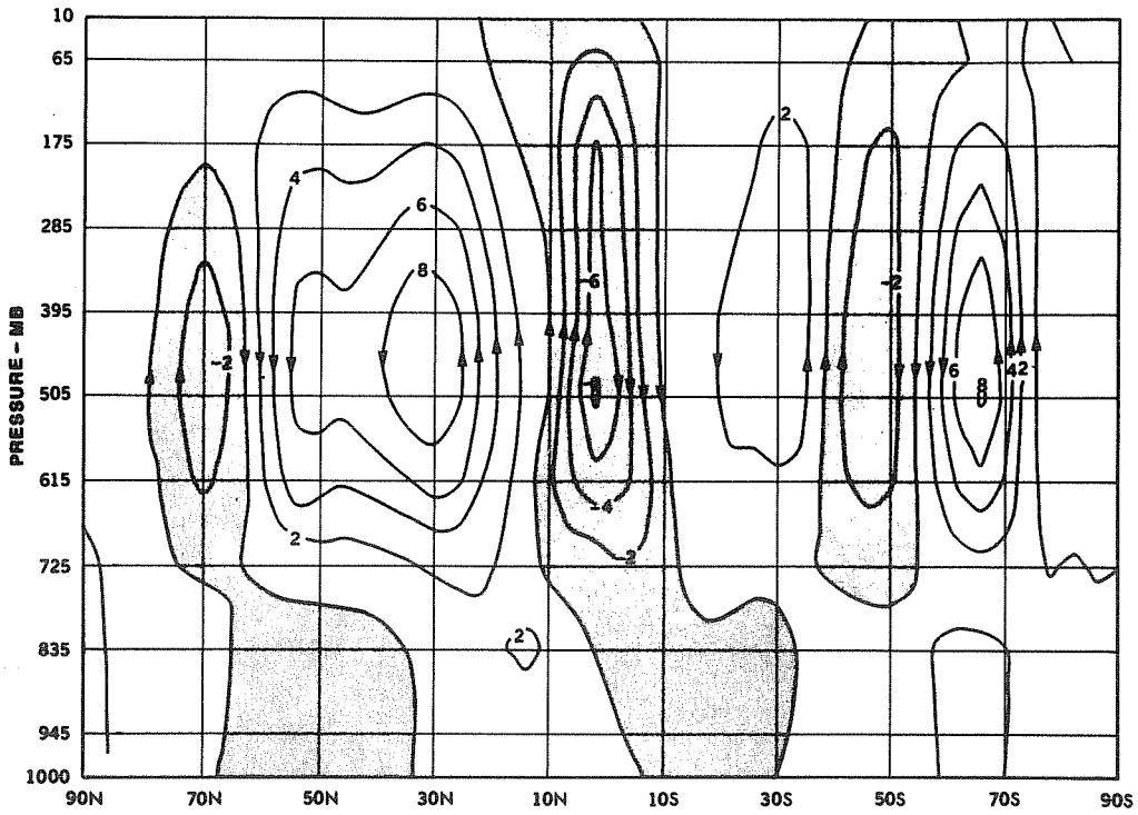
Fig. 4c. Difference of 60 day mean meridional circulation ( 10^{13} gm/sec) averaged between the longitudes 50^{\circ} W and 5^{\circ} W. (From Moura and Shukla, 1981).
