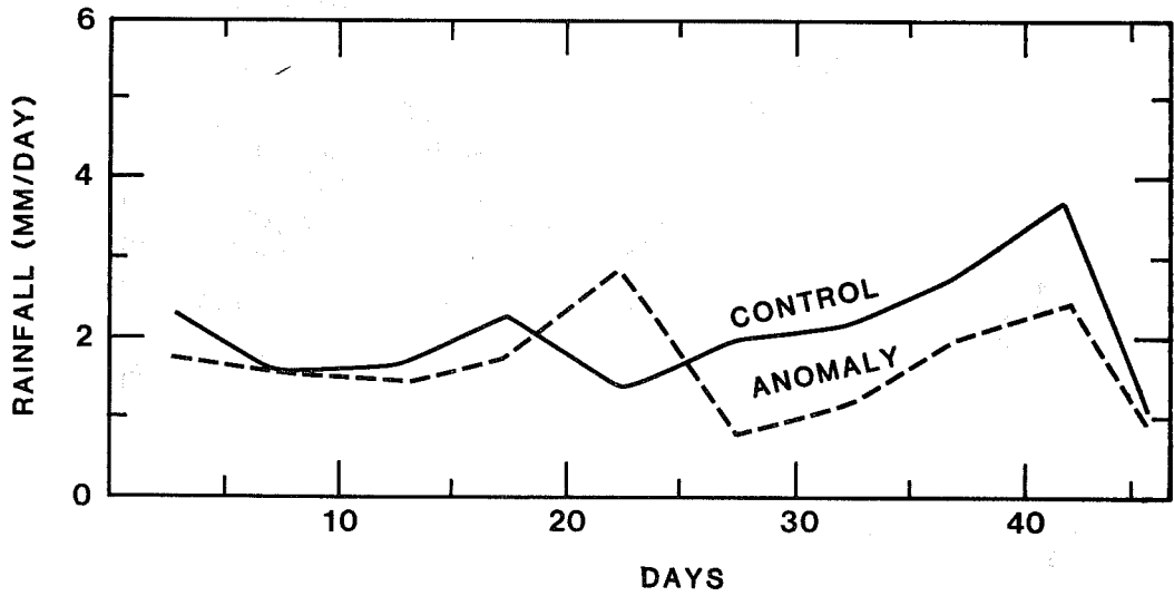
Fig. 7f. Five day average rainfall over northeast Brazil for control and anomaly run.
