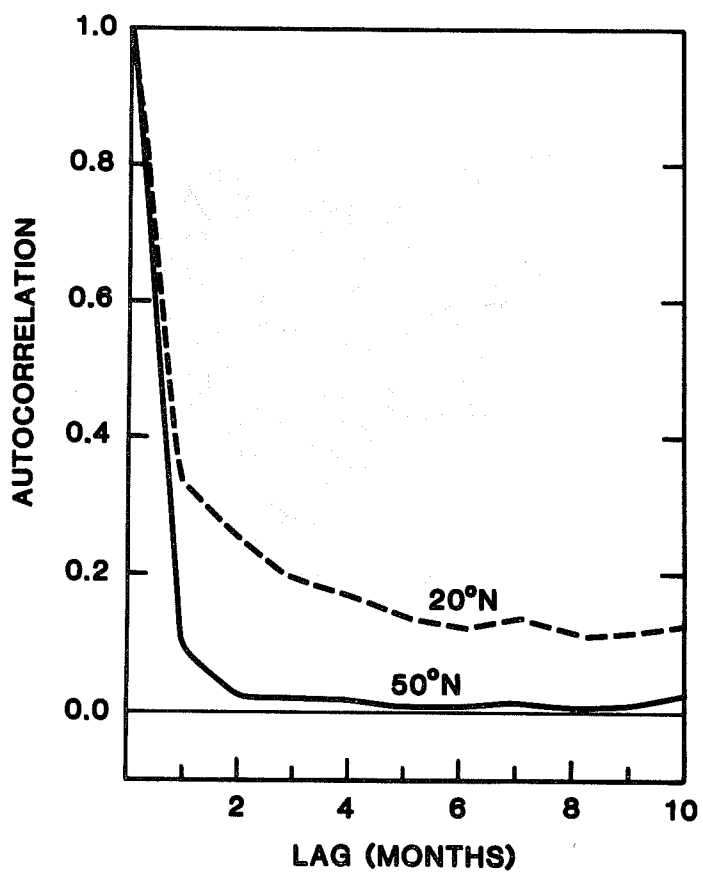
Fig. 11b. Zonally averaged autocorrelation at 20°N and 50°N for monthly mean sea level pressure for the period 1925-77.
