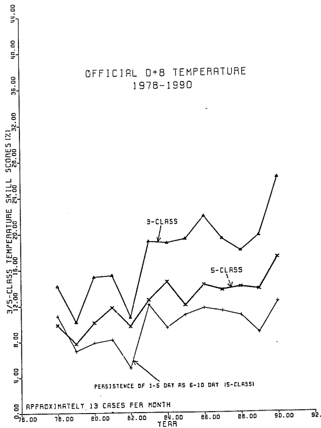
Fig. 6. Annual mean 3-class and 5-class temperature skill scores for the "official" 6-10 day mean predictions for the U.S.
