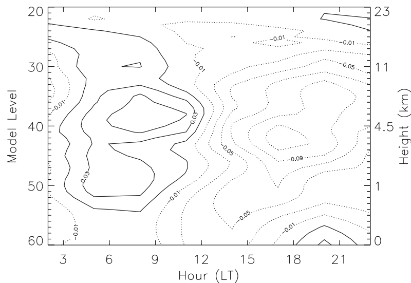
Figure 2 Mean diurnal cycle of omega field for 29-day average from short-term forecasts (in Pa s-1).
