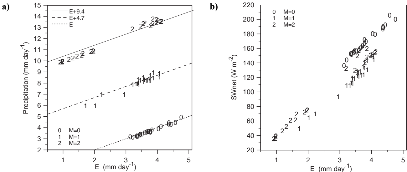
Figure 9a. Scatterplot of 14-day mean precipitation against evaporation for increased mean omega forcing. Figure 9b. As Figure 9a for mean net short-wave radiation.
