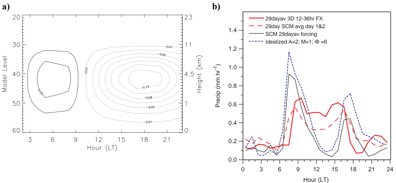
Figure 10a. Idealized omega forcing of SCM for \Phi=6 , M=1 , and A=2 . Figure 10b. Comparison of 29-member ensembles of 3D short term forecasts and SCM runs, with single SCM runs driven by mean GCM forcing and idealized forcing.
