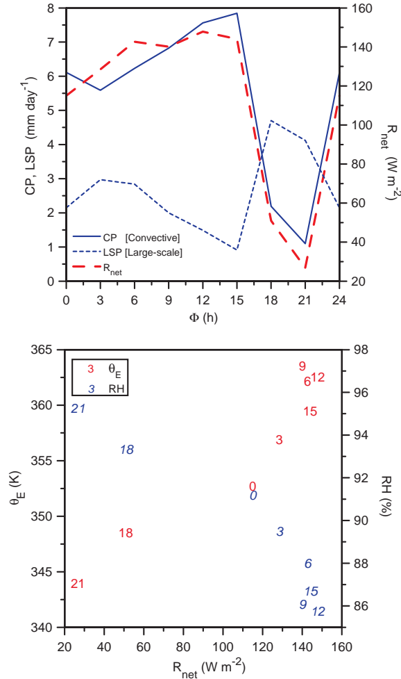
Figure 13 Dependence of convective and large-scale precipitation (mean for days 6-15) and R_{net} on phase (upper panel), and 2-m \theta_E and RH on R_{net} (lower panel).
