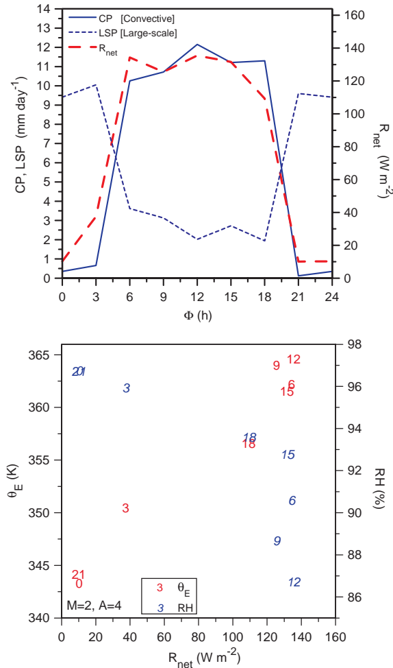
Figure 14 As Figure 13 for M=2 , A=4 .
