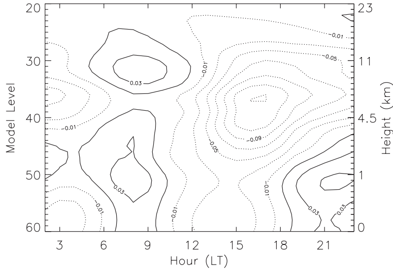
Figure 3 Mean diurnal cycle of omega field for DOY 30-58 from long 'Control' run (in Pa s-1).
