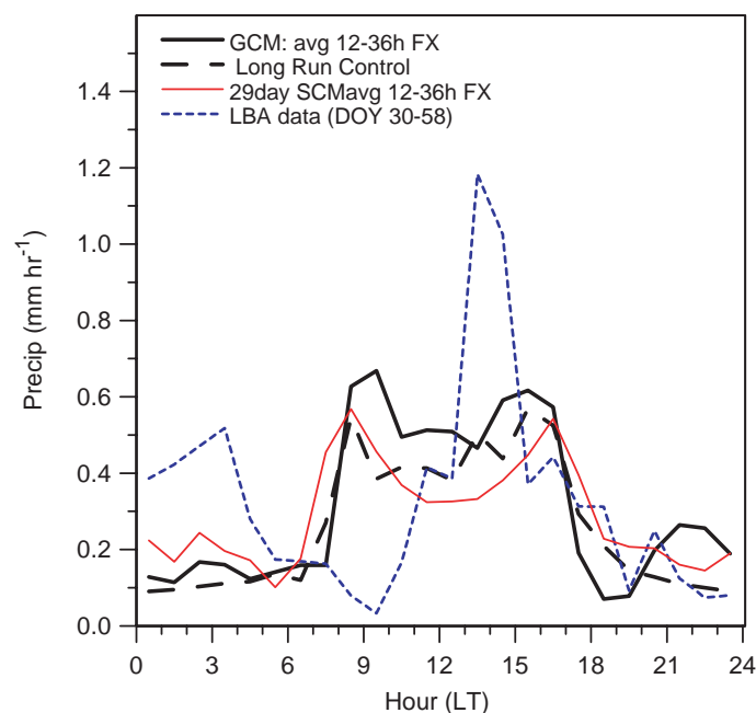
Figure 1 29-day mean diurnal cycle of precipitation from short-term forecasts, long run, and SCM runs using large-scale forcing from the 3-D model.
