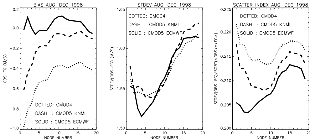
Figure 25: Wind-speed averaged bias, standard deviation and scatter index of inverted winds w.r.t FGAT winds, as a function of node number. Dotted curves are for CMOD4, dashed for CMOD5(KNMI) and solid for CMOD5.
