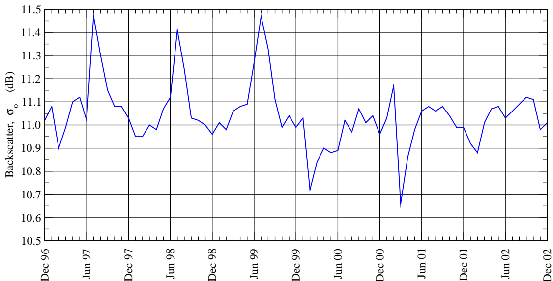
Figure 16: Monthly global mean of ERS-2 RA backscatter coefficient after QC during the period from December 1996 to December 2002.
