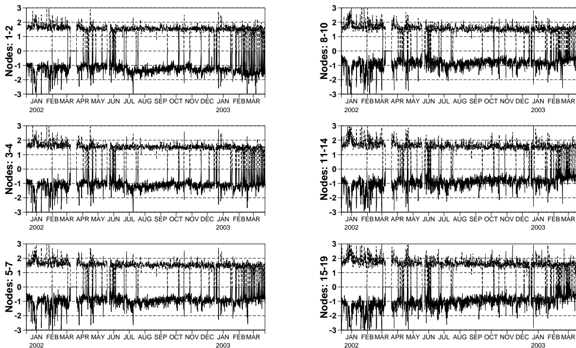
Figure 21: History plot of UWI wind speed versus FGAT
