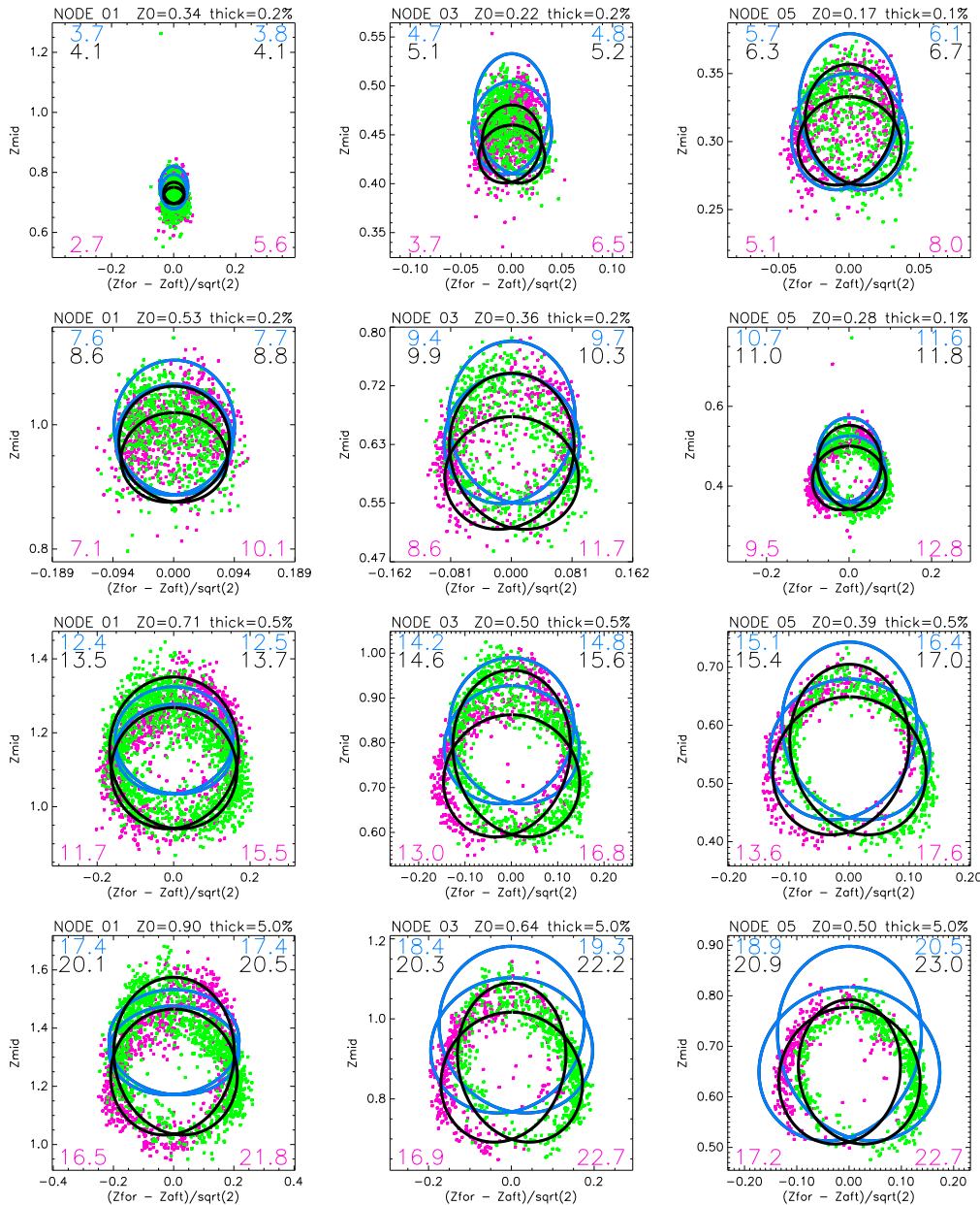
Figure 24: Cone slices for wind values of z_0 = \sigma_0^{0.625} that corresponds to low to high wind speeds, for nodes 1, 3 and 5. Blue curves are cuts of the CMOD4 cone, black curves for CMOD5. Purple points are observed triplets for which the relative wind direction w.r.t. the mid-beam azimuth angle of collocated FGAT winds was between 0 and 180 degrees, green points for directions between 180 and 360 degrees. Numbers within the panels indicate average wind speed plus and minus one standard deviation (left, right respectively) for CMOD4 (blue), CMOD5 (black) and collocated FGAT winds (purple).
