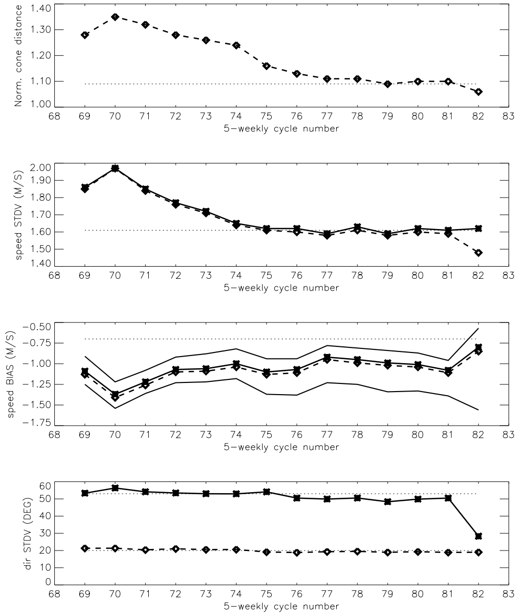
Figure 22: Evolution of the performance of the ERS-2 scatterometer in ZGM averaged over 5-weekly cycles from 12 December 2001 (first data received, cycle 69) to 24 March 2003 (end cycle 82) for the UWI product (solid, star) and de-aliased winds based on CMOD4 (dashed, diamond). Dotted lines represent values for cycle 59 (5 December 2000 to 17 January 2001), i.e. the last stable cycle of the nominal period. From top to bottom panel are shown the normalized distance to the cone (CMOD4 only) the standard deviation of the wind speed compared to FGAT winds, the corresponding bias (for UWI winds the extreme inter-node averages are shown as well), and the standard deviation of wind direction compared to FGAT.
