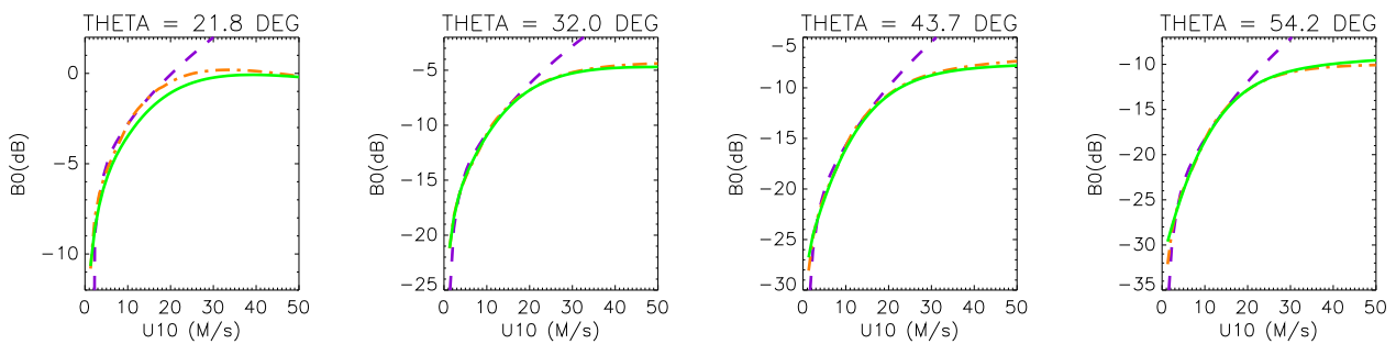
Figure 26: Formulations of the B_0 term for CMOD4 (dashed purple), CMOD5(KNMI) (dash-dotted beige) and CMOD5 (solid green).
