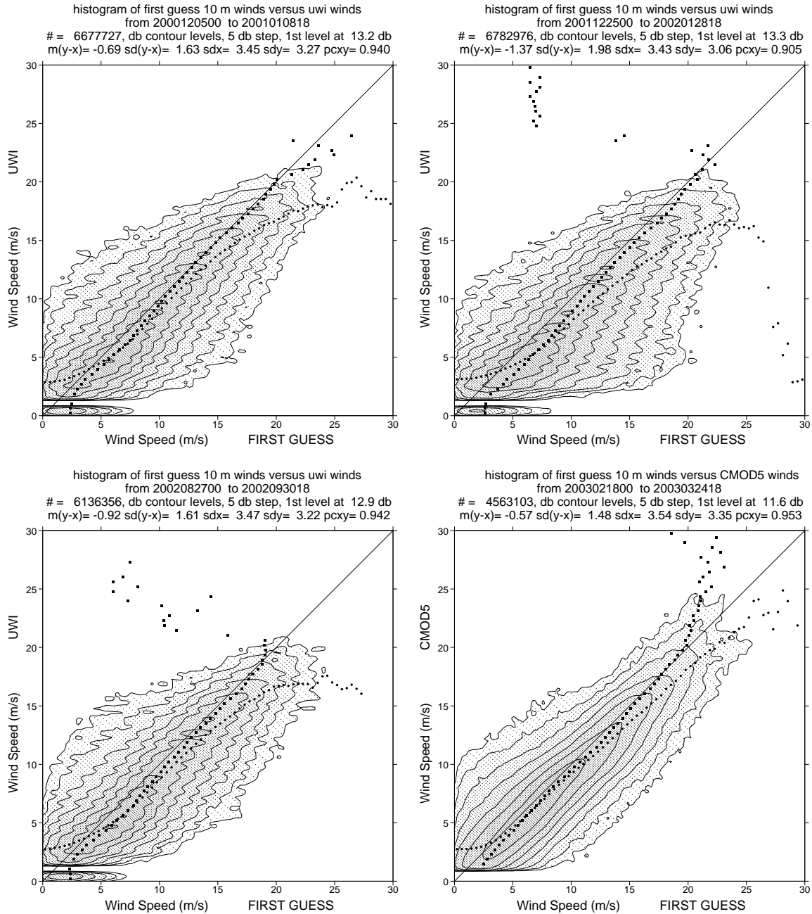
Figure 23: Two-dimensional histogram of FGAT versus UWI wind speeds (top left, cycle 59; top right, cycle 70; bottom left, cycle 77) and of FGAT versus CMOD5 wind speed for cycle 82 (bottom right) for the data kept by the quality control. Circles denote the mean values in the y-direction, and squares those in the x-direction.
