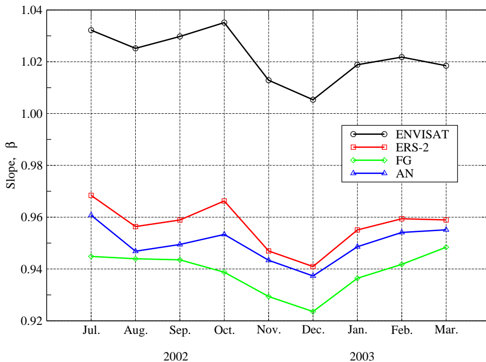
Figure 9: Monthly slope with respect to buoy waves of ENVISAT RA-2 Ku-band, ERS-2 RA, first-guess (FG) and analyzed (AN) wave height during the period from 18 July 2002 to 14 March 2003. (Maximum collocation difference is 5%, wave heights greater than 1 m.)
