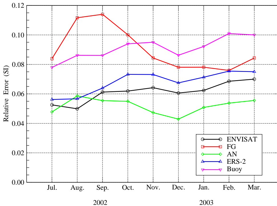
Figure 8: Monthly relative error of ENVISAT RA-2, first-guess (FG), analyzed (AN), ERS-2 RA and buoy wave height during the period from 18 July 2002 to 14 March 2003. (Maximum collocation difference is 5%, wave heights greater than 1 m.)
