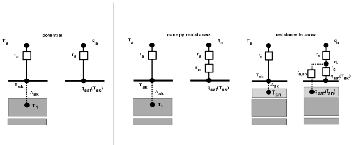
Figure 7.2 Resistance scheme for three categories of coupling. Potential refers to ocean, sea ice and snow on low vegetation; ( Canopy ) resistance to dry low and dry high vegetation, bare soil, and interception reservoir when potential evaporation exceeds the maximum reservoir content; Resistance to snow to snow under high vegetation. For high and low vegetation, an additional canopy resistance r_c is added:
