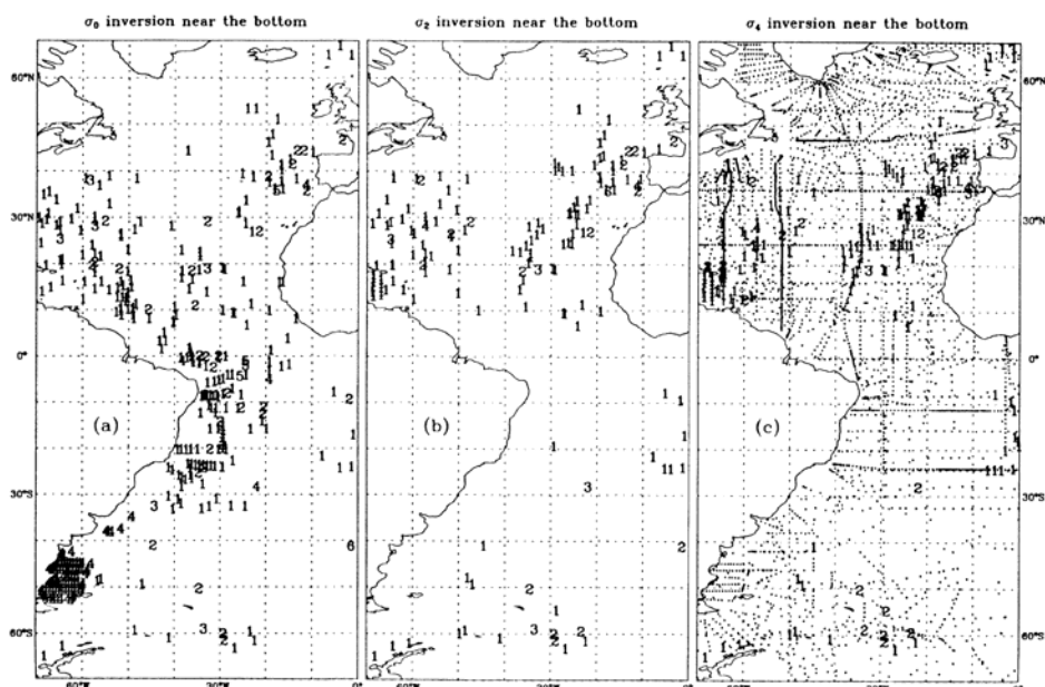
Fig. 7. Potential density inversions in the Atlantic with three different reference pressures: 0dbar (left), 2000 dbar (centre) and 4000 dbar (right), from Read, 1994.
