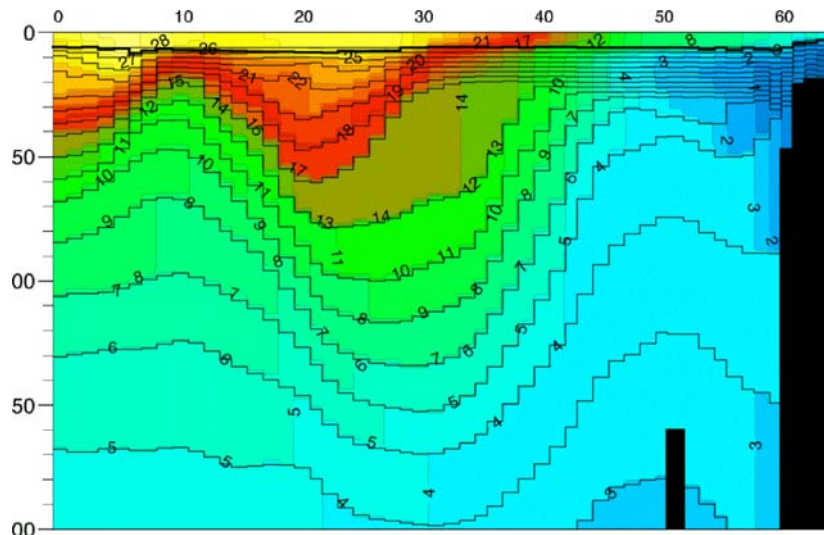
Fig. 5. CHIME coupled model: Temperature section in September in the North Pacific at 180°E. Layer interfaces are shown in black; mixed layer depth is shown by thick line. The transition can be seen from entirely isopycnic layers on the Equator (where there are watermasses present with the lightest densities) to the very north of the Pacific, where many constant-depth levels are deployed. The transition between constant-depth and terrain-following coordinates can also be seen on the continental shelf at the northern end of the section.
