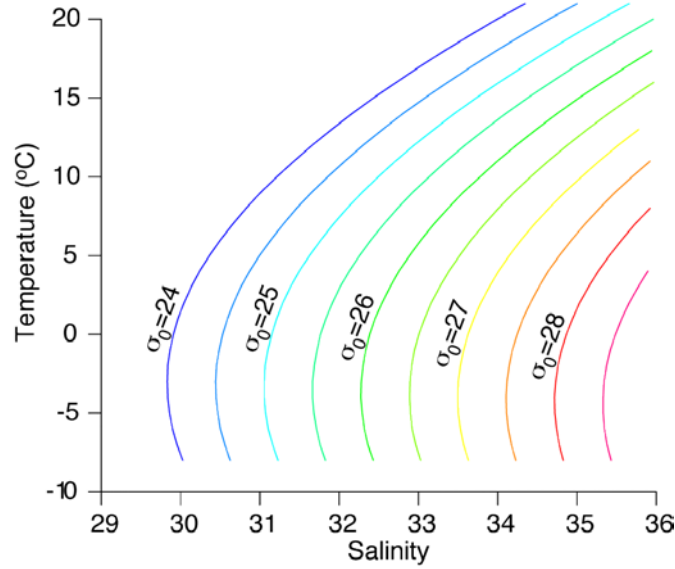
Fig. 3: Friedrich-Levitus equation of state for \sigma_0
