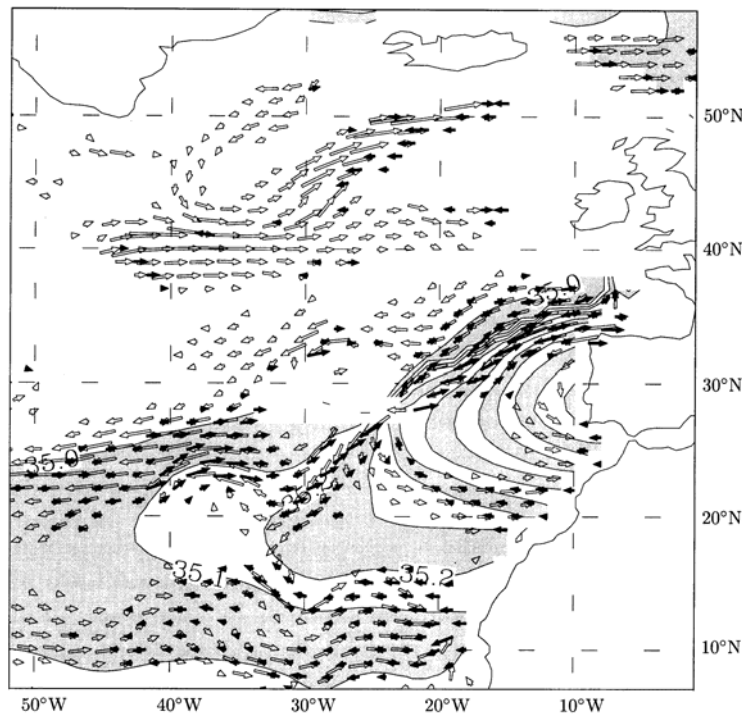
Fig. 8. Thermal wind errors arising from using isopycnal slope. Shaded contours: salinity (interval 0.1 PSU) from Levitus (1994) climatology. Hollow arrows: geostrophic velocity shear on \sigma_0=27.83 . Solid arrows: corrections to this estimate based on slope of \sigma_0 surface to local neutral surface. From S. Sun, Ph.D Thesis.
