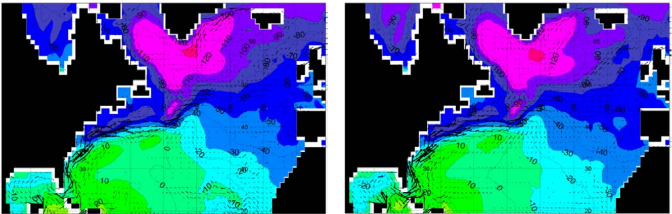
Fig. 10. Mean surface elevation and surface layer velocity in CHIME coupled model: at 20 years (left) and at 80 years (right).
