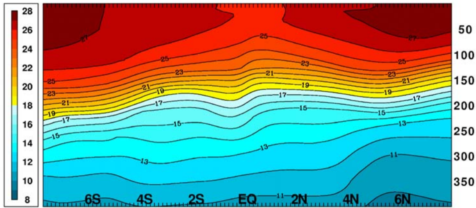
Fig. 9(b). Temperature cross-section at 135°W from 1/12° Pacific HYCOM
