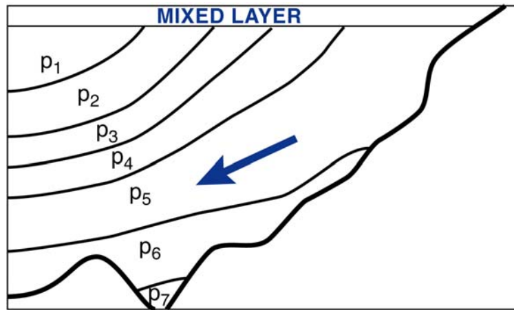
Fig. 2: Schematic of isopycnic model
