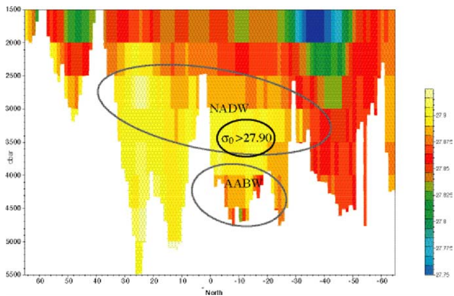
Fig. 6. Potential density ( \sigma_0 ) at 30°W (September; Levitus 1992)
