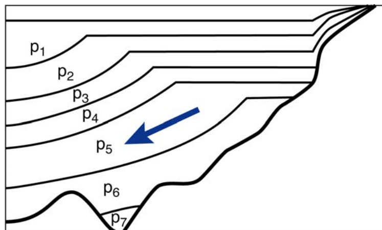
Fig. 4: schematic of isopycnic model
