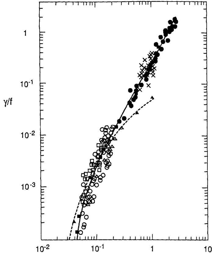
Figure 3.1 Comparison of theoretical growth rates with observations by Plant (1982) (full line): Miles' theory; (full dots): parametrization of Miles' theory (3.3); dashed line: the fit by Snyder et al. (1981) .
