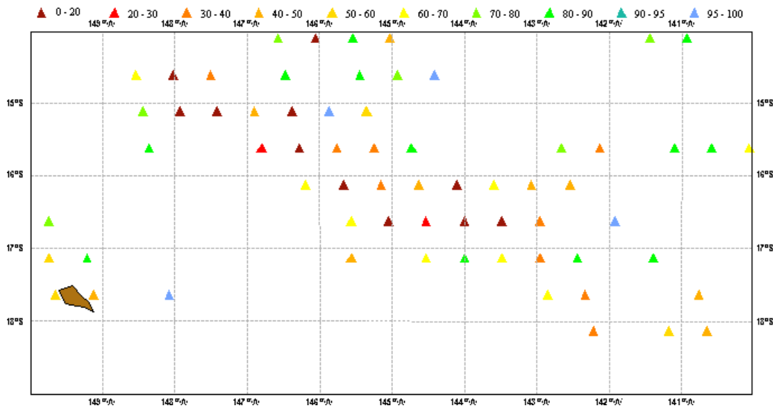
Figure 5.5 Percentage of the wave energy that is allowed propagates northwards for the lowest frequency bin (~ 0.035 Hz).
