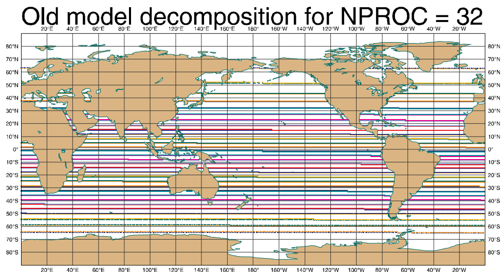
Figure 6.4 1-D decomposition of the WAM model 0.5^\circ irregular lat-long grid for 32 processors. The different colour lines indicate grid points sharing information with neighbouring PE's.
