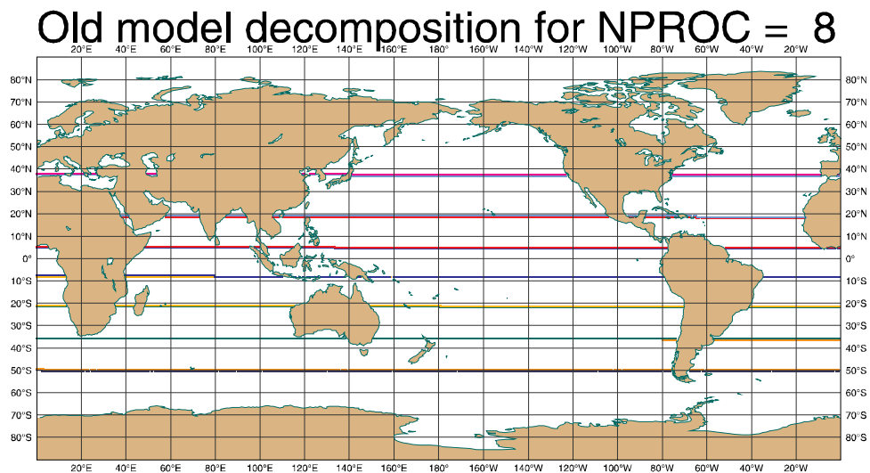
Figure 6.3 1-D decomposition of the WAM model 0.5^\circ irregular lat-long grid for 8 processors. The different colour lines indicate grid points sharing information with neighbouring PE's.
