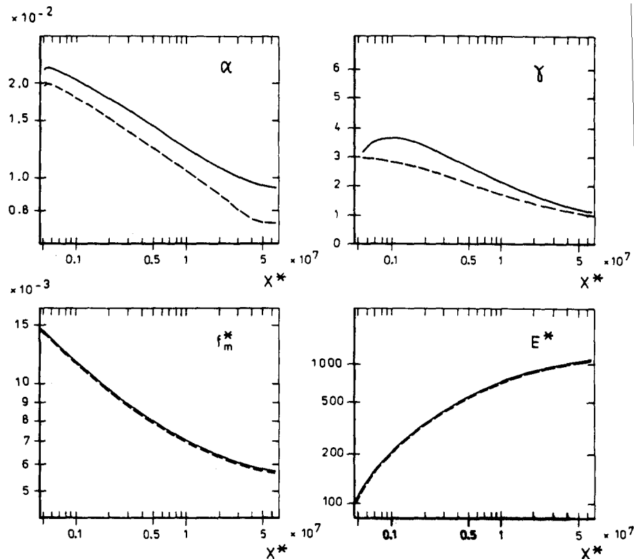
Figure 3.3 Comparison of fetch-growth curves for spectral parameters computed using the exact form and the discrete interaction approximation of S_{nl} . All variables are made dimensionless using u_* and g .
