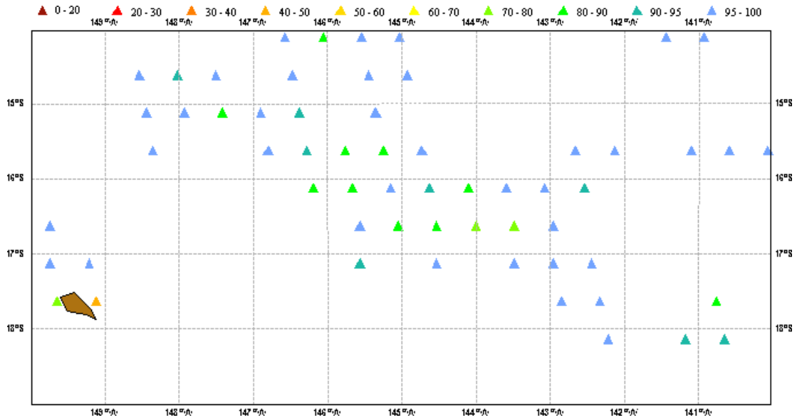
Figure 5.6 Percentage of the wave energy that is allowed propagates northwards for the highest frequency bin (~ 0.55 Hz).
