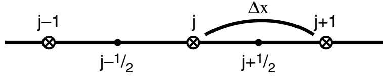
Figure 3: Definition of grid points for first-order upwinding scheme.
