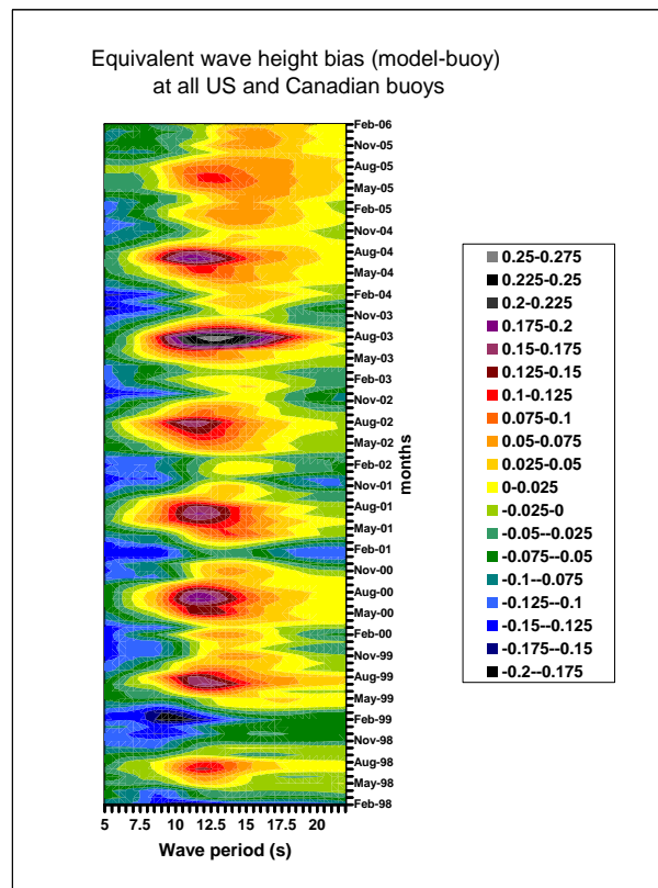
Figure 6: Spectral bias (model-buoy) at all US and Canadian buoys for the period February 1998 until February 2006.
