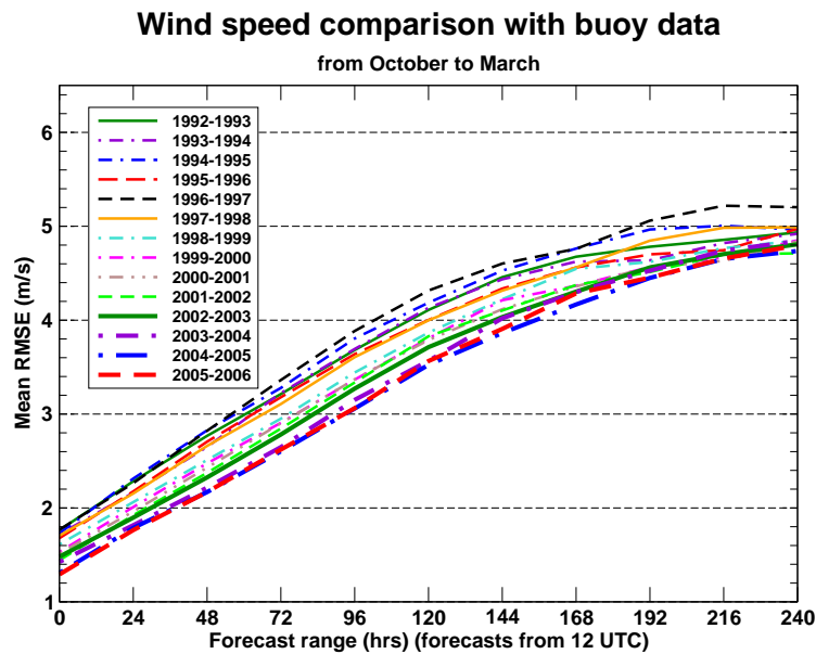
Figure 4: Verification of analyzed and forecast surface wind speeds against buoy observations.
