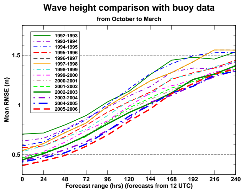
Figure 5: Verification of analyzed and forecast significant wave height against buoy observations.
