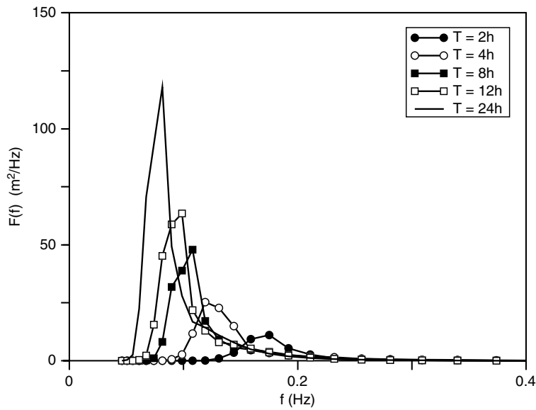
Figure 1: Evolution in time of the one-dimensional frequency spectrum according to the ECWAM model.
