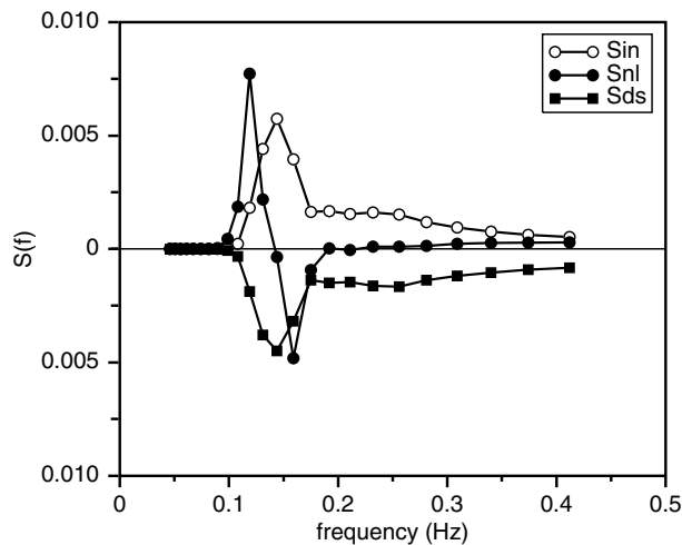
Figure 2: The energy balance for young windsea at a duration of 4 h.
