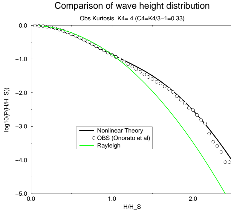
Figure 7: Comparison of theoretical and observed [64] wave height distribution. For reference, the linear Rayleigh result is shown as well.
