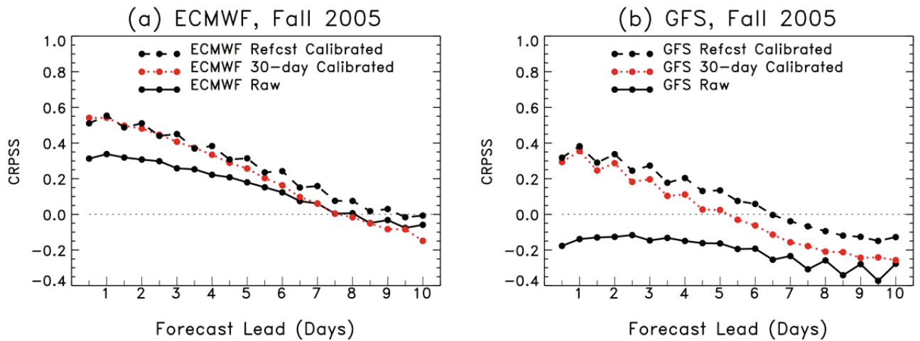
Fig. 6 Comparison of CRPSS using 30-day and 20-year training data sets for the period 1 October – 1 December 2005. (a) ECMWF data, (b) GFS data.
