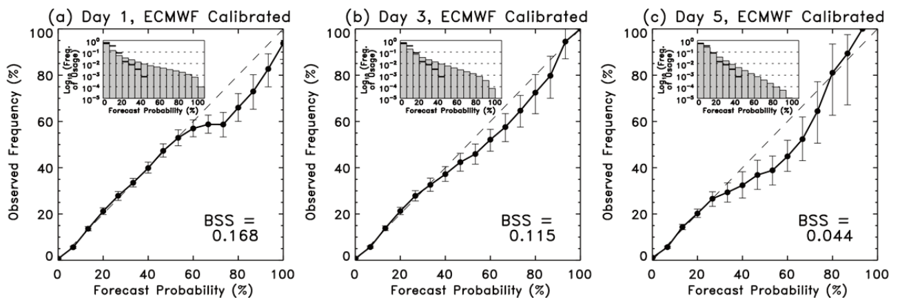
Fig. 9 As in Fig. 7, but for calibrated ECMWF forecasts.
