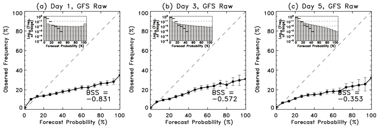
Fig. 8 As in Fig. 7, but for GFS raw forecasts.
