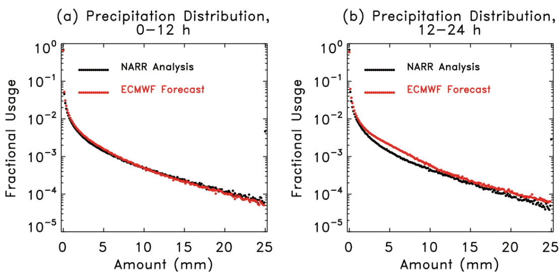
Fig. 12 Distribution of the fractional usage of precipitation amounts from the North American Regional Reanalysis and ECMWF raw forecasts for (a) 0 -12 hour forecasts, and (b) 12-24 hour forecasts.
