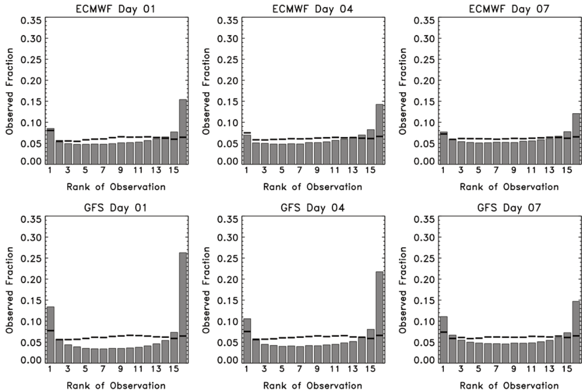
Fig. 3 Rank histograms for 2-meter temperatures from ECMWF and GFS ensembles at 1, 4, and 7 days lead. Histograms denote the raw ensemble and solid lines the histogram derived from the pdf of the calibrated forecasts.
