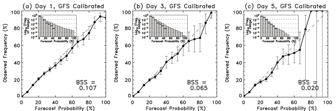
Fig. 10 As in Fig. 7, but for calibrated GFS forecasts.
