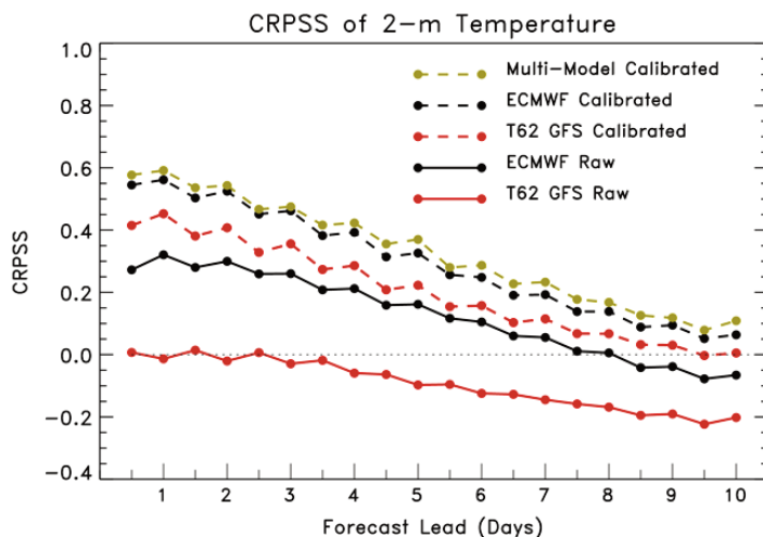
Fig. 4 (a) CRPSS of surface temperature forecasts with and without calibration, and (b) CRPSS including bias-corrected ensemble forecasts.
