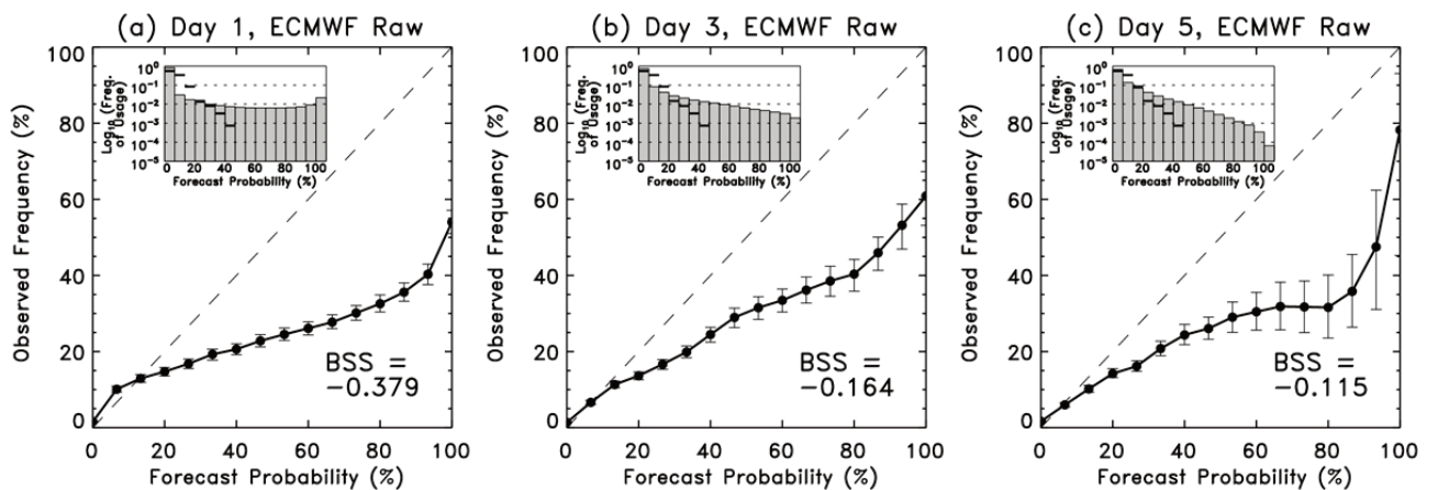
Fig. 7 Reliability of 5-mm ECMWF raw forecasts at 1, 3, and 5-day leads. Overplotted confidence intervals provide 5th and 95th percentiles of determined through block bootstrap resampling techniques. Inset histogram denotes frequency of forecast usage of each probability bin. Solid lines overlaid on histogram denote the climatological frequency of usage of each probability bin.
