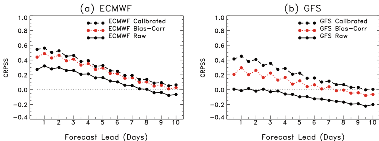
Fig. 5 CRPSS including bias-corrected ensemble forecasts for (a) ECMWF forecasts, and (b) GFS forecasts.
