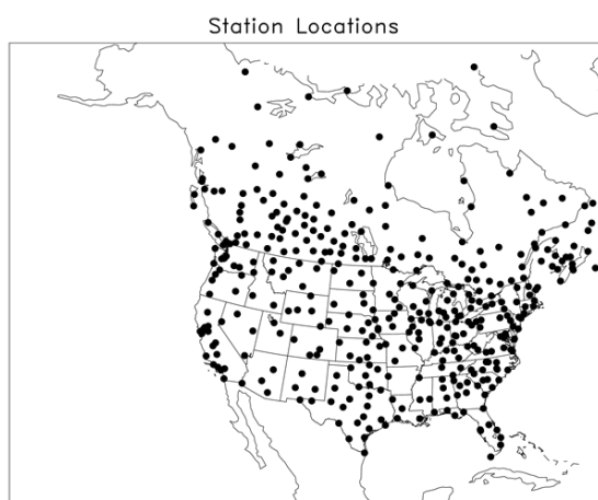
Fig. 1 Station locations for the verification of 2-meter temperature forecasts.
