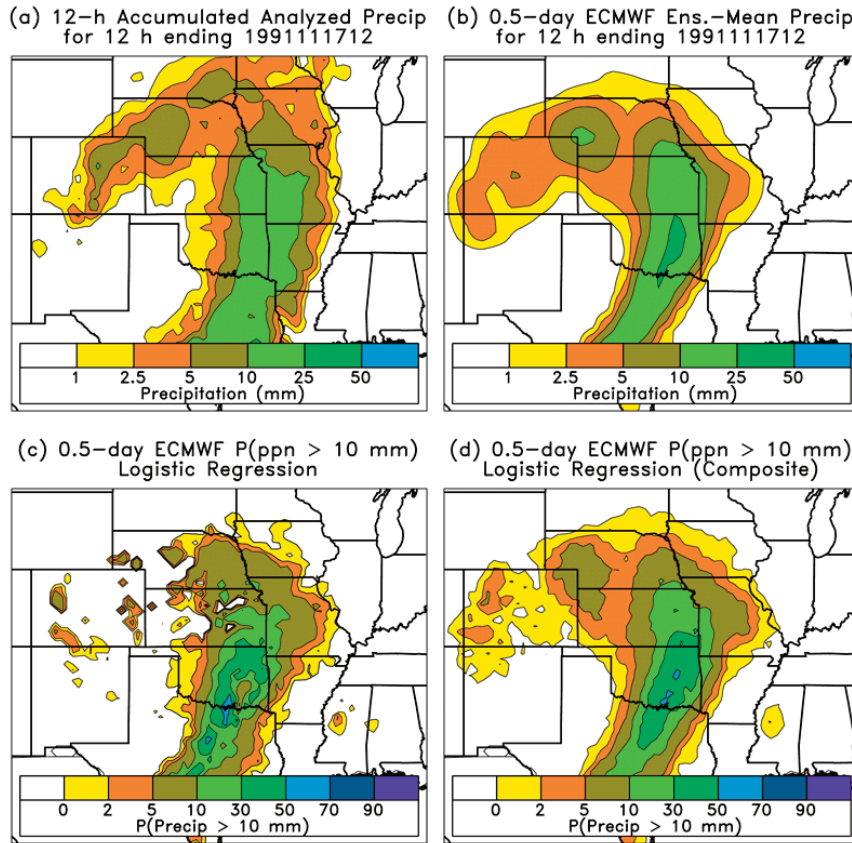
Fig. 2 (a) NARR precipitation analysis of 12-h accumulated precipitation for the 12-hourly period ending 1200 UTC 17 November 1991. (b) 0-12 hour ECMWF ensemble-mean forecast of accumulated precipitation. (c) Probability of greater than 10 mm precipitation in this period using a logistic regression where each grid point's data is treated independently. (d) As in (c), but where the logistic regression training data includes forecasts and observations from 10 other locations that have similar observed precipitation climatologies for this day of the year.
