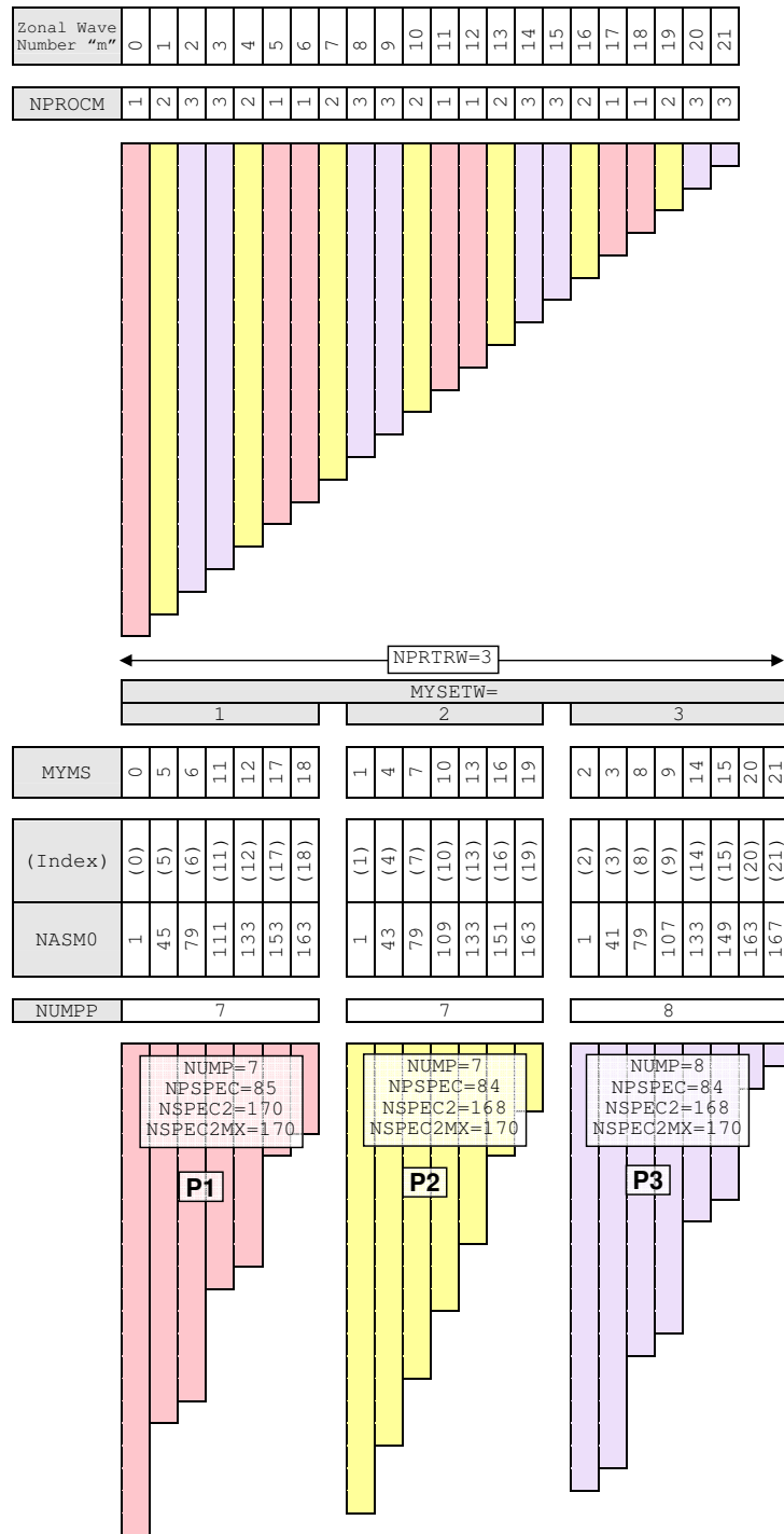
Figure 2.15 Distribution of zonal wave numbers (T21 spectral triangle).
