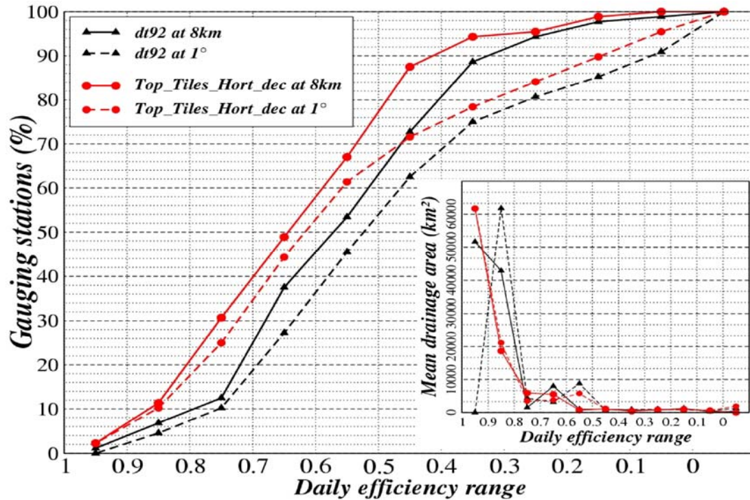
Figure 2: Cumulative efficiency (Nash criterion) distribution of daily river discharges simulated at 88 gauging stations distributed over the Rhône river basin. All hydrological simulations are driven by observed atmospheric forcings either at a 8km (solid lines) or 1^\circ (dashed lines) horizontal resolution and coupled to the MODCOU river routing model. ISBA-SGH (in red) is compared to the standard ISBA model (in black). From Decharme and Douville 2006
