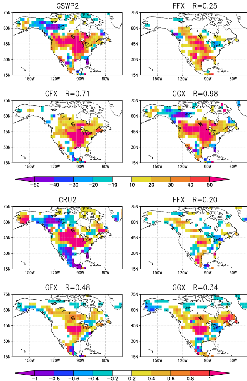
Figure 5: Observed (GSWP-2 and CRU2 climatologies) and simulated (ensemble mean) differences (1993 minus 1988) in summer soil moisture ( \text{kg/m}^2 , upper panels) and precipitation ( \text{mm/day} , lower panels) over North America. Three ensembles driven by observed monthly SST are compared using free soil moisture (FFX, no nudging), GSWP-2 initial conditions of soil moisture (GFX, nudging until the end of May), GSWP-2 boundary conditions of soil moisture (GGX, nudging until the end of September). R denotes the spatial anomaly correlation coefficient between observations and simulations. Adapted from Conil et al. 2008.
