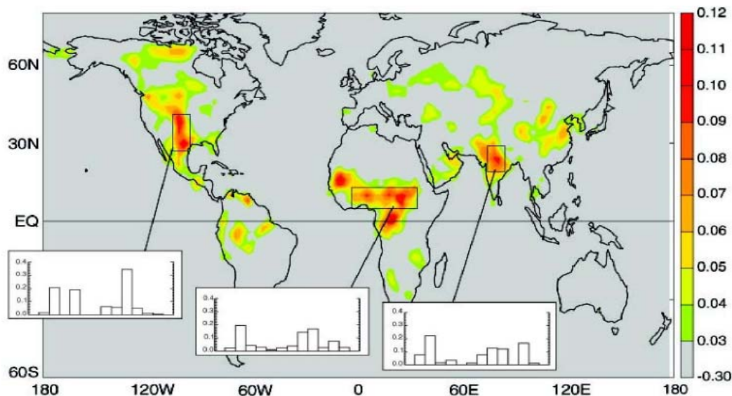
Figure 7: Land-atmosphere coupling strength diagnostic (dimensionless index describing the impact of soil moisture on precipitation) for boreal summer averaged across 12 models. Areal averaged coupling strengths for the 12 individual models over the outlined hotspot regions. From Koster et al. 2004.
