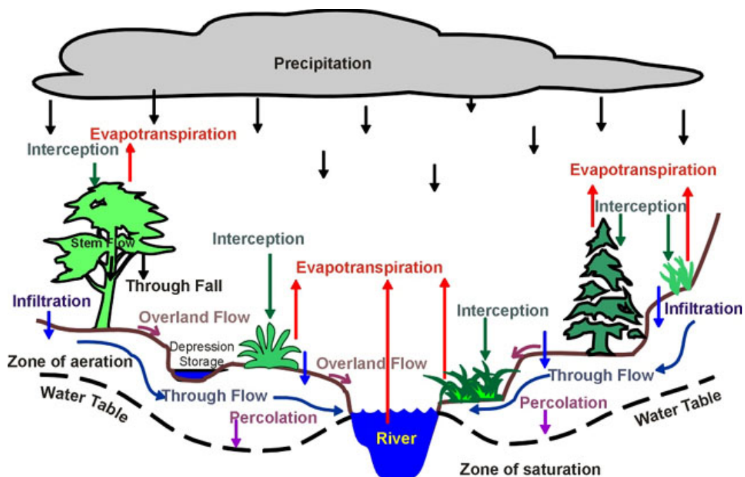
Figure 1: The main sources of subgrid hydrological variability accounted for in the ISBA-SGH land surface model of CNRM (Decharme and Douville 2006): precipitation, orography and vegetation.
