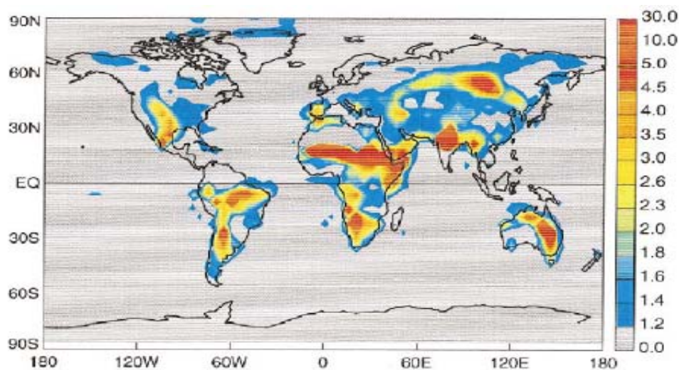
Figure 4: Amplification of annual precipitation variance due to land-atmosphere feedback in the NASA GEOS-ARIES atmospheric GCM, estimated as the ratio of variance between two ensembles of simulations driven by observed SSTs, but using interactive versus climatological land surface boundary conditions (that is climatological land surface evaporation efficiency). From Koster et al. 2000.
