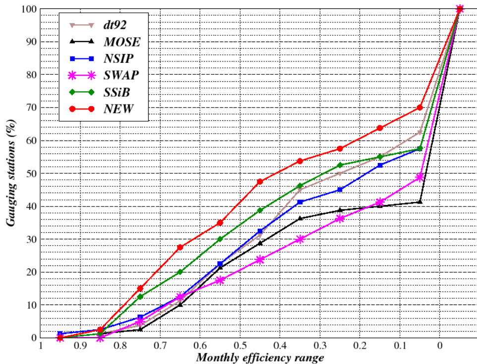
Figure 3: Cumulative efficiency (Nash criterion) distribution of monthly river discharge simulated from 1986 to 1995 at 80 gauging stations distributed over the largest (>100000 km 2 ) world's river basins. Six land surface models are compared : ISBA-SGH (NEW) and ISBA-standard (dt92), as well as four other LSMs having contributed to the international GSWP-2 intercomparison project (B3 atmospheric forcing). Runoff from all simulations has been converted into river discharge using the TRIP river routing model (Oki and Sud 1998). From Decharme and Douville 2007.
