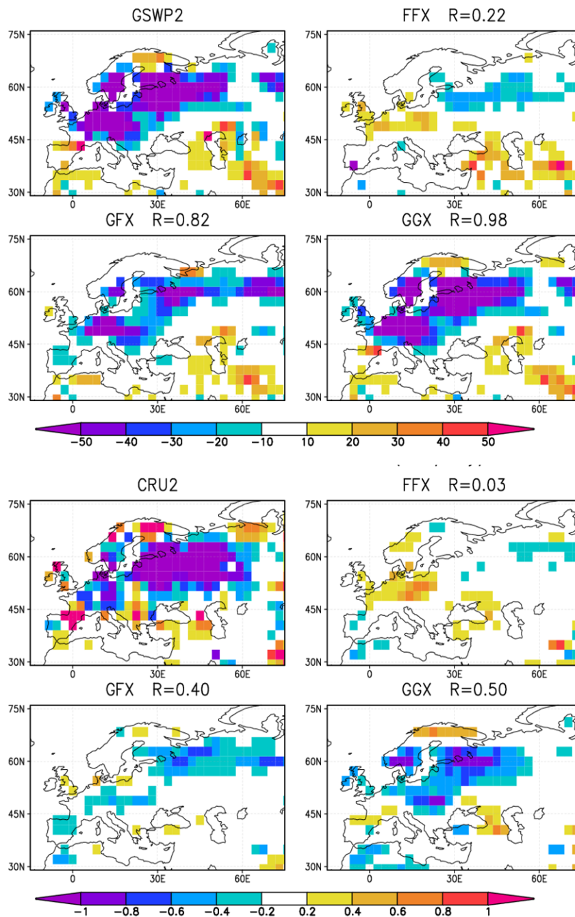
Figure 6: Observed (GSWP-2 and CRU2 climatologies) and simulated (ensemble mean) differences (1992 minus 1987) in summer soil moisture ( \text{kg/m}^2 , upper panels) and precipitation ( \text{mm/day} , lower panels) over Europe. Three ensembles driven by observed monthly SST are compared using free soil moisture (FFX, no nudging), GSWP-2 initial conditions of soil moisture (GFX, nudging until the end of May), GSWP-2 boundary conditions of soil moisture (GGX, nudging until the end of September). R denotes the spatial anomaly correlation coefficient between observations and simulations. Adapted from Conil et al. 2008.
