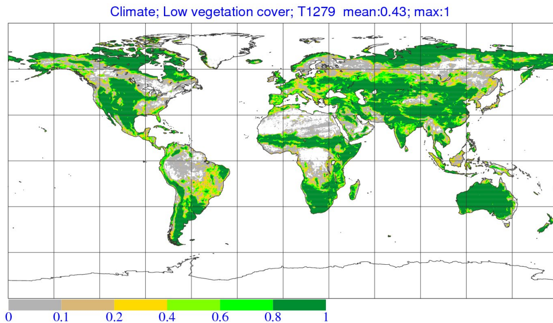
Figure 11.9 Fractional cover of low vegetation.
