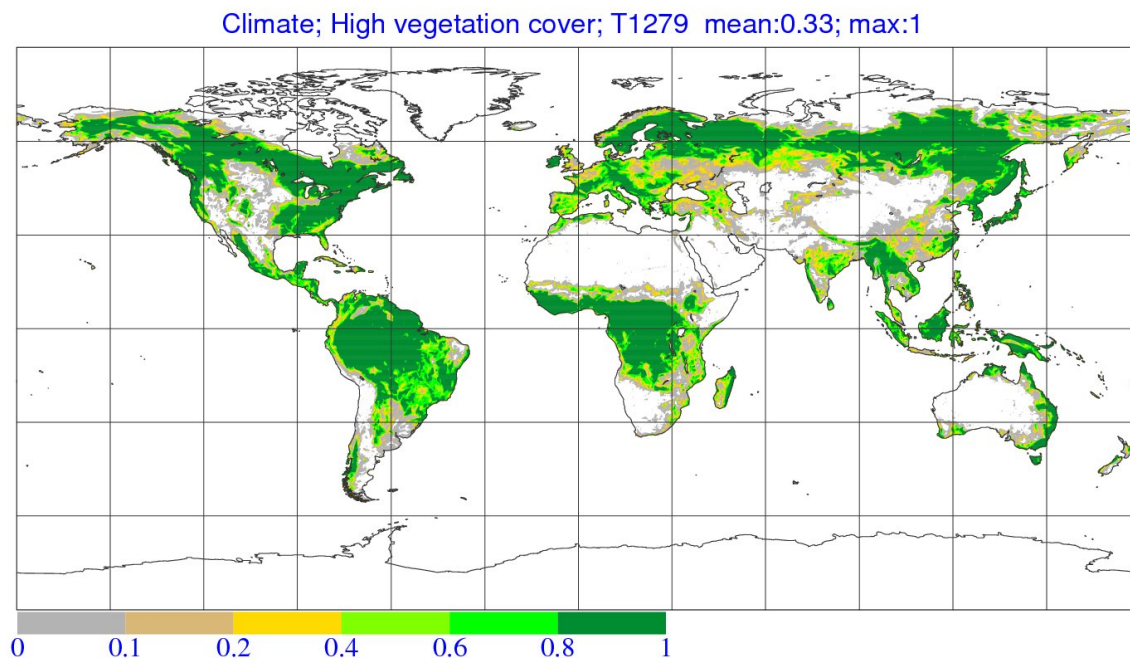
Figure 11.10 Fractional cover of high vegetation.
