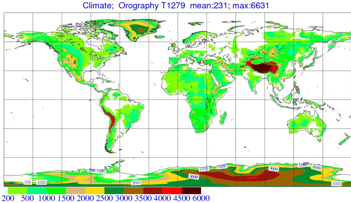
Figure 11.1 Orography at T1279 resolution.
