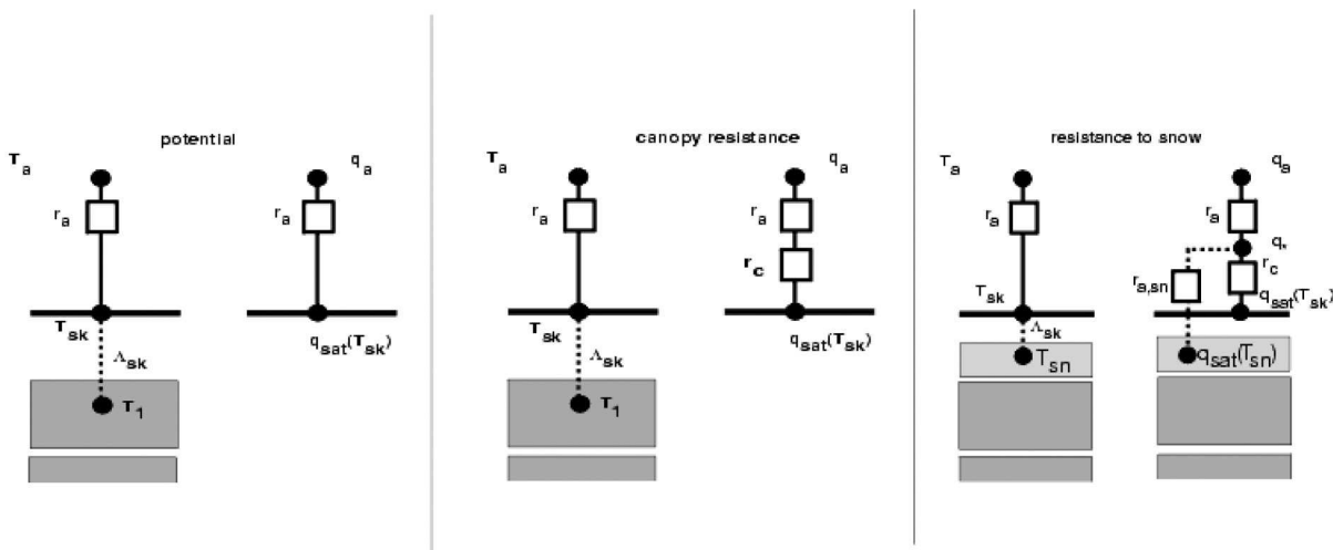
Figure 8.2 Resistance scheme for three categories of coupling. Potential refers to ocean, sea ice and snow on low vegetation; ( Canopy ) resistance to dry low and dry high vegetation, bare soil, and interception reservoir when potential evaporation exceeds the maximum reservoir content; Resistance to snow to snow under high vegetation.
