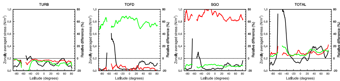
Figure 4: Zonal averages of the magnitude of \tau_{tot} ( N/m^2 ) and of its components for the CTL experiment (black, scale on left). The green and red curves, scale on right, show the relative change of \tau_{tot} and of its components in the experiments H-TOFD and H-BLOCK with respect to the CTL. The zonal averages are computed as in Fig. 2.
