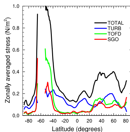
Figure 2: Zonal averages of the magnitude of \tau_{tot} ( N/m^2 ) and of its components from the TURB, TOFD and SGO schemes for the CTL experiment. These zonal averages are computed from monthly means of daily surface stress magnitude (derived from the first 24 hours of the daily 00UTC forecasts performed for February 2014), include only land grid cells and were smoothed using a 5 degrees running mean.
