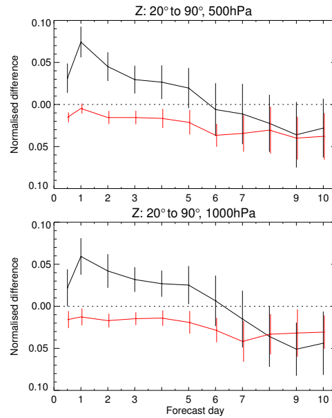
Figure 9: Relative difference of root mean square error (RMSE) of 500hPa and 1000 hPa geopotential height, between the H-TOFD (black), respectively H-BLOCK (red), and the CTL forecasts, as a function of lead time. When error bars do not cross the zero-line the performance of the respective experiment is significantly worse/better (95 % interval) than the CTL. For both the experiments and the CTL forecasts the RMSE was computed with respect to the analysis from which the forecasts started. A positive difference in RMSE indicates a deterioration of the model performance in the experiment with respect to the CTL.
