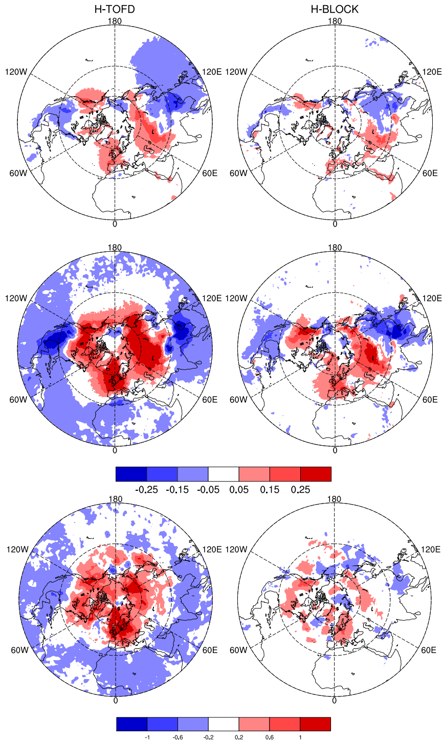
Figure 7: Mean change in surface pressure (hPa) in the experiments H-TOFD (left) and H-BLOCK (right) with respect to the CTL, at leadtime 6 (top) and 24 (middle) and 120 (bottom) hours of the daily 00UTC forecasts performed for February 2014.
