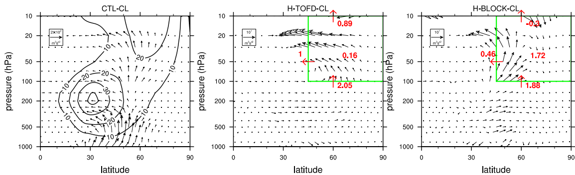
Figure 12: Left: EP-flux (arrows) and zonal mean zonal wind (contours, m/s) in the CTL-CL experiment for the 30 DJF seasons (1984-2014). Center/right: Change in EP-flux (arrows) in H-TOFD-CL, respectively H-BLOCK-CL with respect to the CTL-CL experiment over the 30 DJF seasons. For clearer visualisation the EP flux arrows have been scaled by the relative ranges of the two axes of the plot ( 3.14 radians by 10^5 Pa). The visibility of vectors in the stratosphere has been further enhanced by using a scaling factor proportional to the square-root of pressure and by applying a magnifying factor (of 3) above 100hPa. A budget for resolved wave driving is presented for the stratospheric box between 100 and 10 hPa and between 45 and 90 N. Red numbers across the box represent differences of EP fluxes integrated over the box boundaries between the H-TOFD-CL/H-BLOCK-CL and the CTL-CL experiment, while the red numbers in the box represent the differences in time- and area-mean momentum deposition, or EP flux divergence, associated with the resolved waves (all wavenumbers) within the box ( 10^4 \text{ kgms}^{-4} ).
