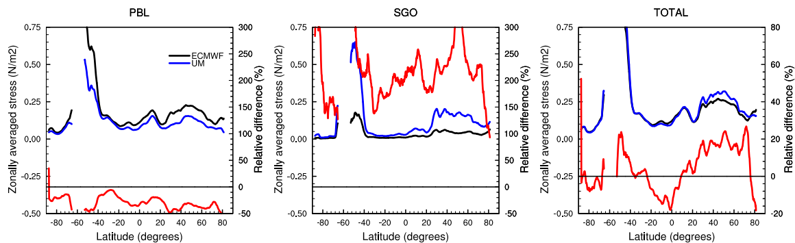
Figure 1: Zonal averages of the magnitude of the total subgrid surface stress \tau_{tot} ( N/m^2 ) and of its components for ECMWF (black, scale on left) and UM (blue, scale on left), from the results submitted for the WGNE Drag project for January 2012, and relative difference between UM and ECMWF (red, scale on right). For comparison with the results from the WGNE Drag project, the magnitude of the stress used to construct the zonal averages is computed in this plot only from monthly mean diurnal averages of the u and v components of the surface stress (derived from the first 24 hours of the daily 00UTC forecasts). The zonal averages include only land grid cells and were smoothed using a 5 degrees running mean.
