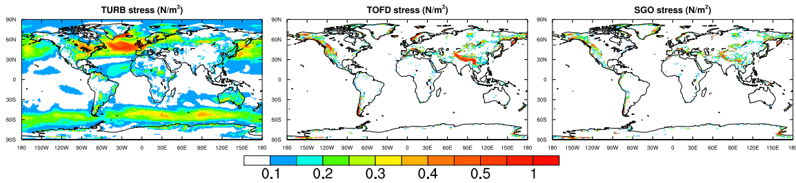
Figure 3: Magnitude of the surface stress due to the TURB, TOFD and SGO schemes ( N/m^2 ) for the CTL experiment. These fields represent monthly means of the daily surface stress magnitude, derived from the first 24 hours of the daily 00UTC forecasts performed for February 2014.
