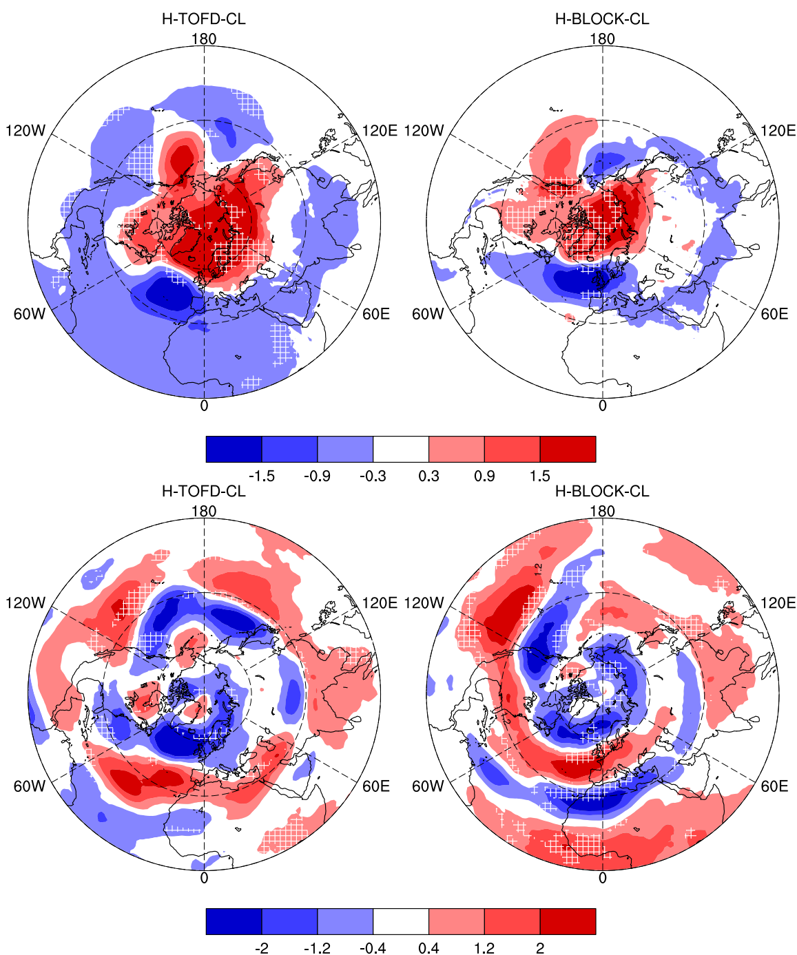
Figure 10: Mean change in surface pressure (hPa) (top row) and zonal wind at 200hPa (m/s) (bottom row) in H-TOFD-CL and H-BLOCK-CL with respect to the CTL-CL experiment over the 30 DJF seasons (1984-2014). The horizontal white pattern (gridded areas) indicate 90 (95) % statistical significance according to a paired t-test.
