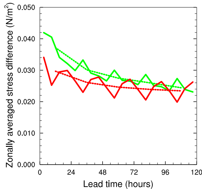
Figure 6: Time evolution of the monthly mean differences in the magnitude of \tau_{tot} ( N/m^2 ) between the H-TOFD (green), respectively H-BLOCK (red) and the CTL experiment during the first five days of the forecasts performed for February 2014, integrated over the Himalaya area showed in Fig. 5. Full lines indicated 6-hourly averages, and dash lines indicate diurnal averages of the difference in the magnitude of \tau_{tot} . The forecasts start at 00UTC.
