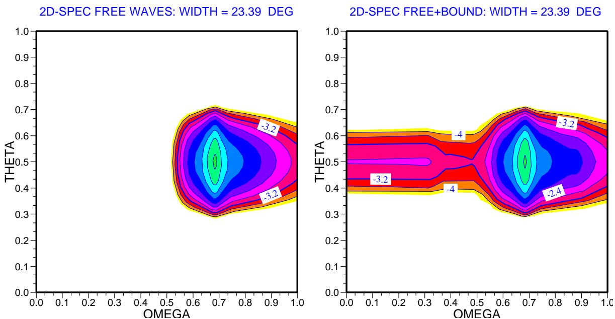
Figure 9.4 Two-dimensional frequency-direction spectrum for a windsea with a width of 23°, but now calculated on a reduced spectral grid (reduction factor = 2).
