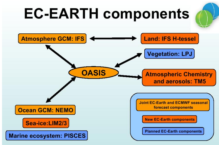
Figure 1: Components used in the EC-Earth model
