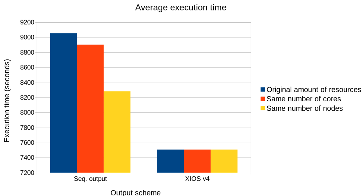
Figure 31: Comparison test with additional computational resources of the execution time of two different output schemes. In blue they are using the original amount of resources, in orange they are using the same amount of cores, and in yellow they are using the same amount of nodes
