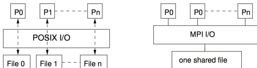
Figure 5: Common writing strategies: on the left side the strategy for writing multiple files and on the right side the strategy for writing one file (Reproduced from [18])
