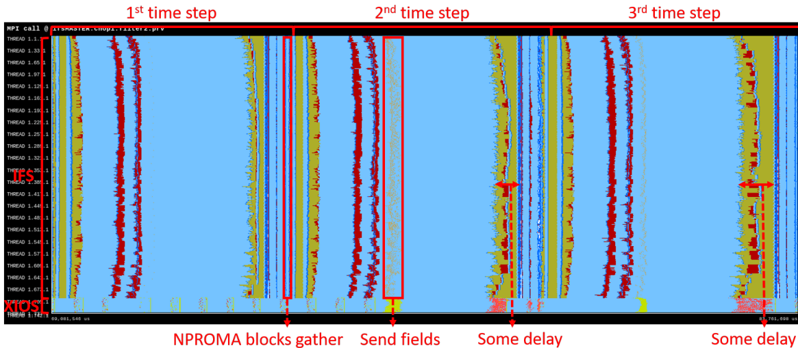
Figure 24: Trace with three IFS time steps once optimized
