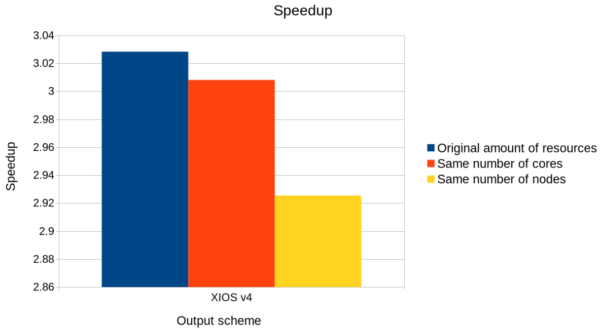
Figure 34: Speedup of XIOS v4 against the sequential output scheme with additional computational resources and GRIB to netCDF conversion cost. In blue the original amount of resources, in orange the same amount of cores, and in yellow the same amount of nodes
