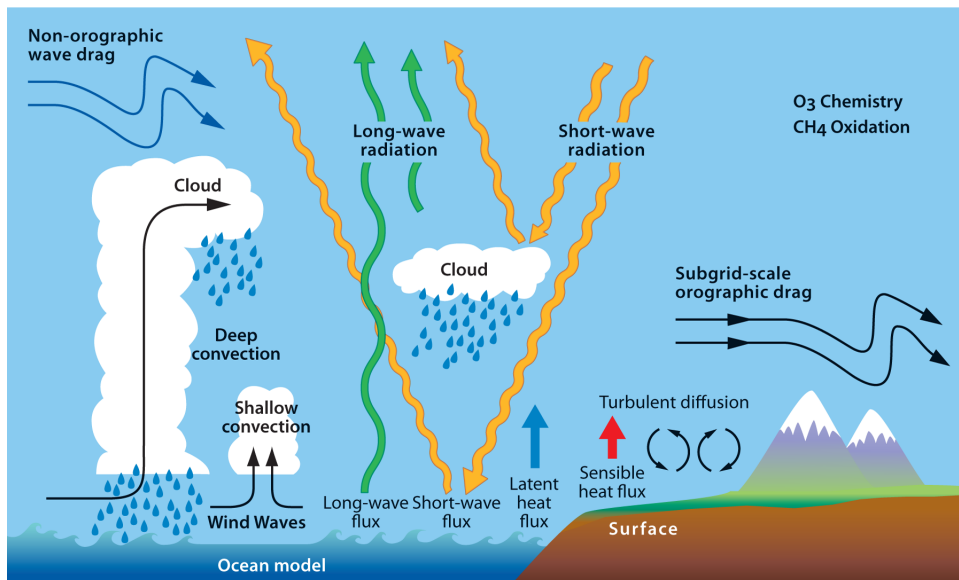
Figure 9: Overview of the unresolved physical processes in the atmosphere (Reproduced from [34])
