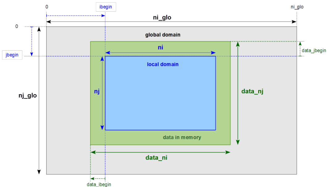
Figure 15: Basic variables to describe the global domain and a subdomain (Reproduced from [14])
