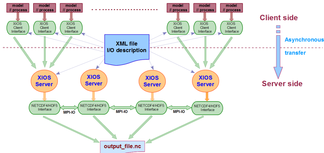
Figure 11: Overview of the XIOS architecture. Model processes are communicated with the XIOS servers using asynchronous MPI messages. All the framework is configured using an XML file (Reproduced from [14])
