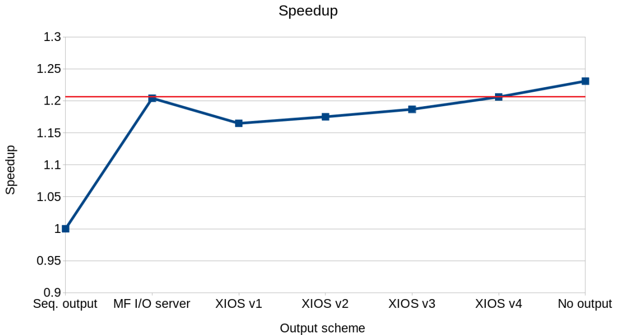
Figure 28: Comparison of the speedup of different output schemes
