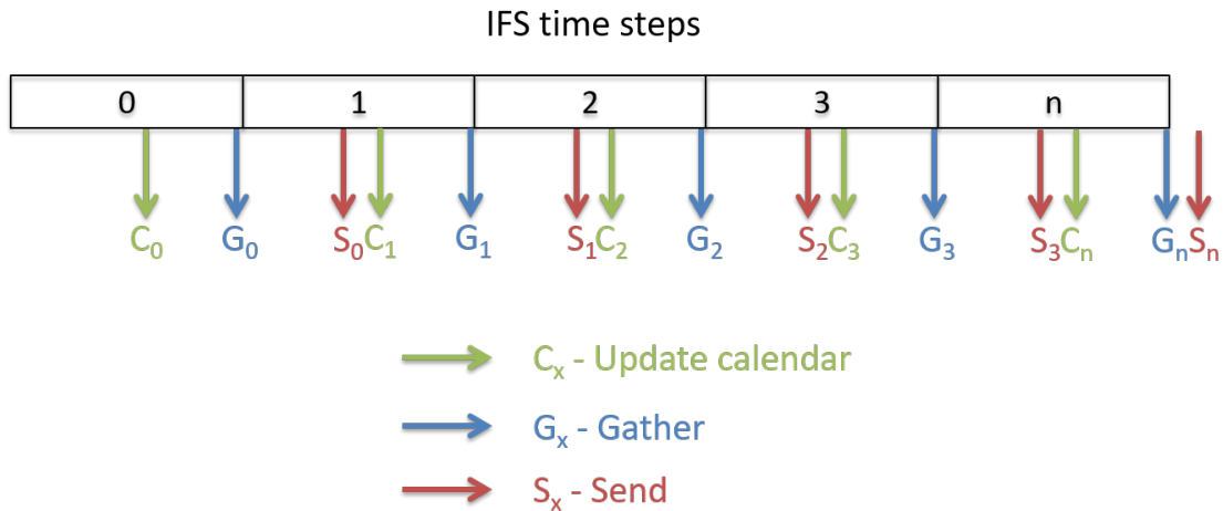
Figure 23: Optimized output scheme developed for IFS. The three needed steps to output data are split: the update calendar is performed in the middle of the time step; the NPROMA blocks gather is maintained at the end of the time step; and the send fields is delayed to the next time step
