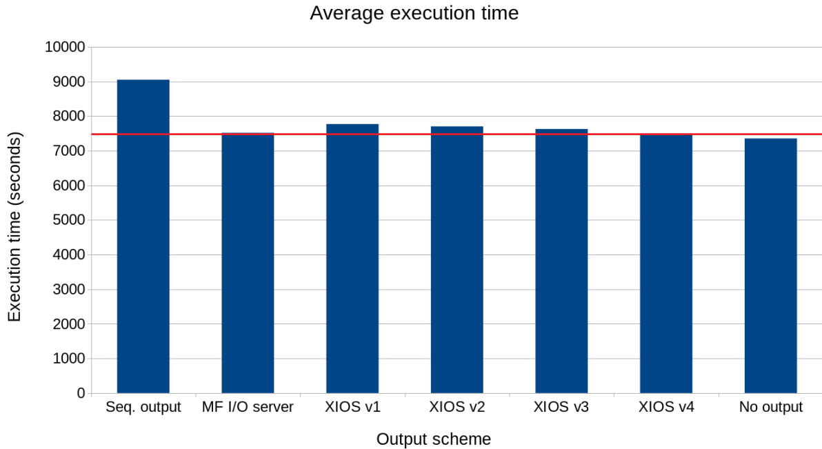
Figure 27: Comparison of the execution time of different output schemes
