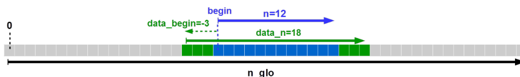
Figure 13: Basic variables to describe an axis (Reproduced from [14])
