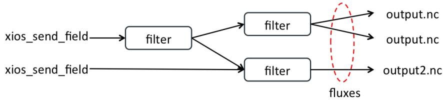
Figure 16: Example of a workflow applying filters to fields
