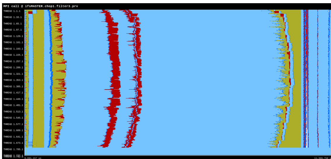
Figure 20: Example of a trace with MPI call events. It shows a complete regular time step of an IFS-XIOS execution. Timeline is on the x axis and MPI processes on the y axis.
