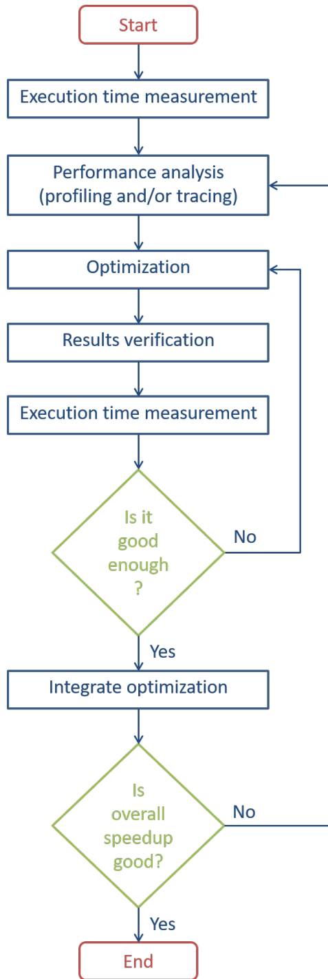
Figure 19: Performance analysis and optimization flowchart
