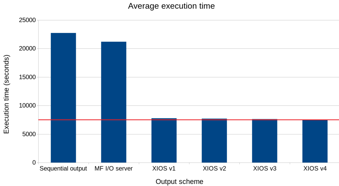
Figure 29: Comparison of the execution time of different output schemes, where both sequential output and MF I/O server have the additional cost of converting GRIB to netCDF files
