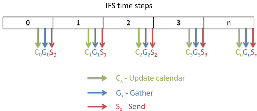
Figure 18: Output scheme developed for IFS: all three steps, update calendar, NPROMA blocks gather and send fields are sequentially executed at the end of and output time step
