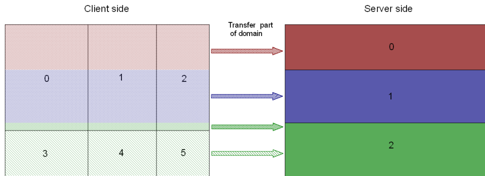
Figure 12: Example of XIOS data distribution between clients and servers (Reproduced from [14])
