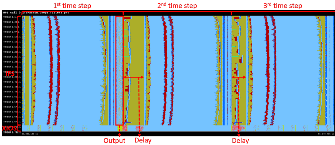
Figure 22: Trace with three IFS time steps
