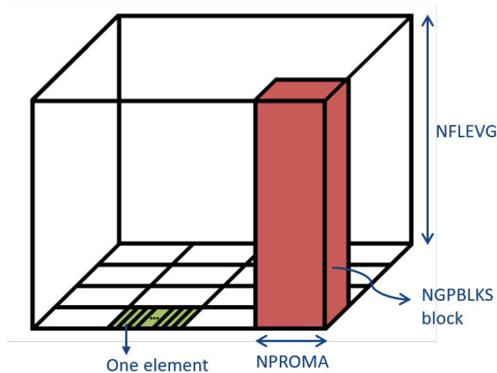
Figure 10: NPROMA blocking strategy used for IFS data arrays. For each NPROMA block, IFS iterates over all elements (NPROMA) of each vertical level (NFLEVG) and for each field (NFIELDS)
