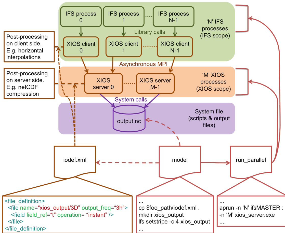
Figure 17: Scheme of the IFS-XIOS integration. It overviews how the different parts are interconnected.
