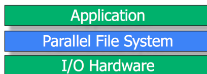
Figure 4: Sequential I/O stack traditionally used by HPC applications (Reproduced from [15])
