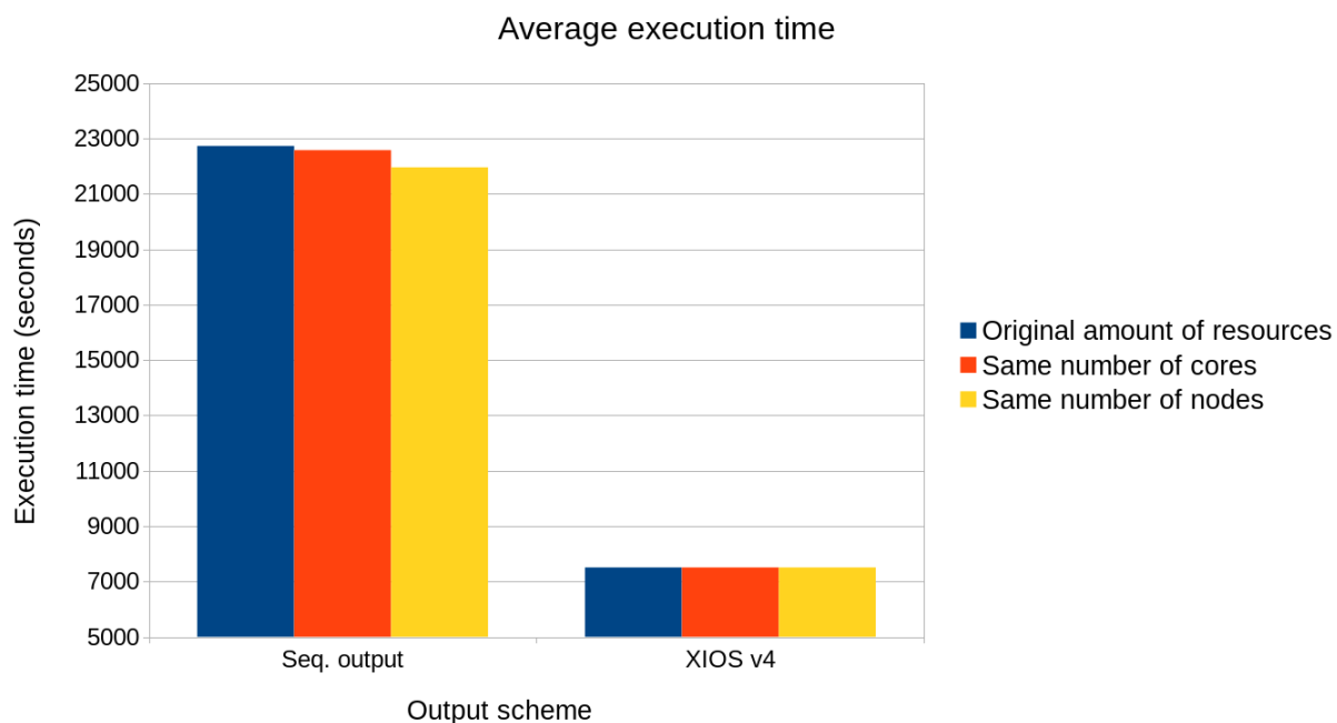
Figure 33: Execution time comparison test with additional computational resources and GRIB to netCDF conversion cost of two different output schemes. In blue they are using the original amount of resources, in orange they are using the same amount of cores, and in yellow they are using the same amount of nodes
