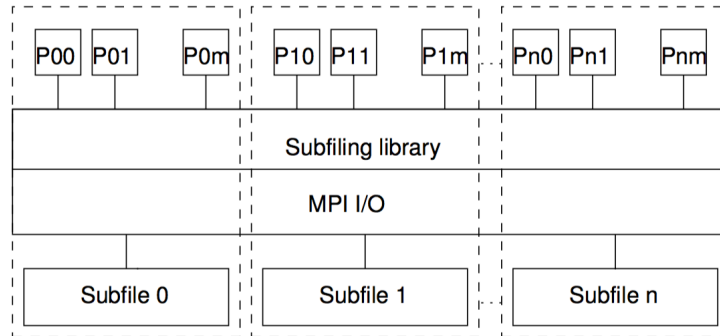
Figure 6: Intermediate I/O strategy: processes are grouped in subsets to share a file (Reproduced from [18])
