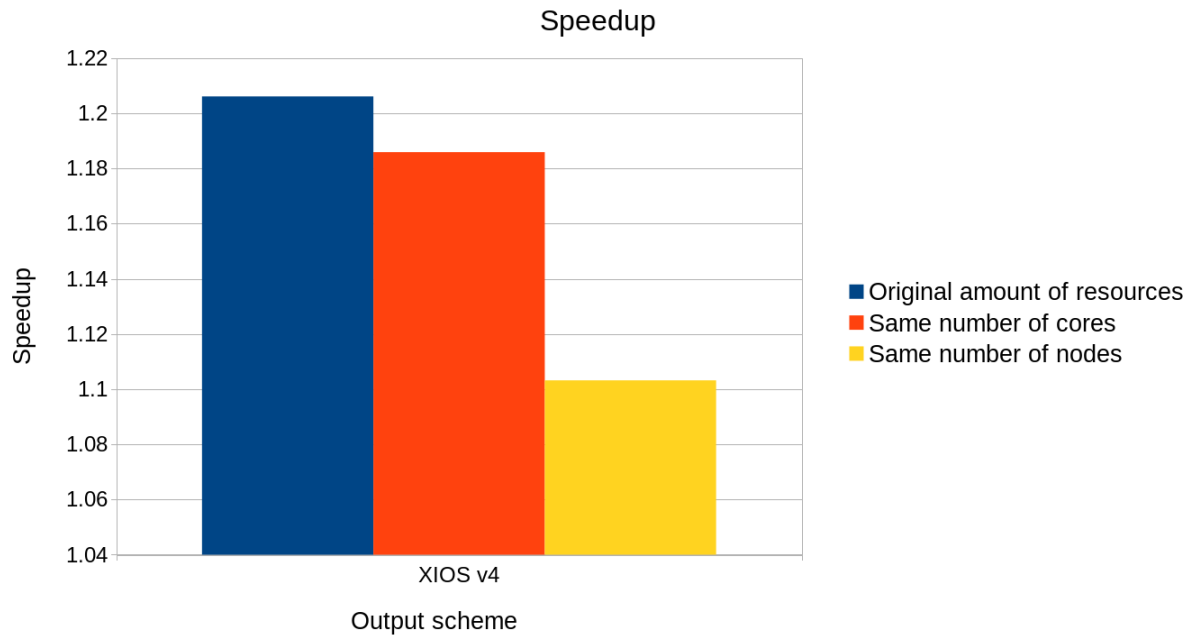
Figure 32: Speedup of XIOS v4 against the sequential output scheme with additional computational resources. In blue the original amount of resources, in orange the same amount of cores, and in yellow the same amount of nodes
