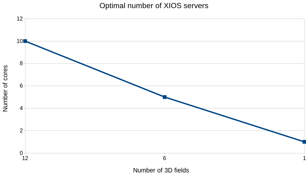
Figure 26: Optimal number of XIOS servers in function of the output size
