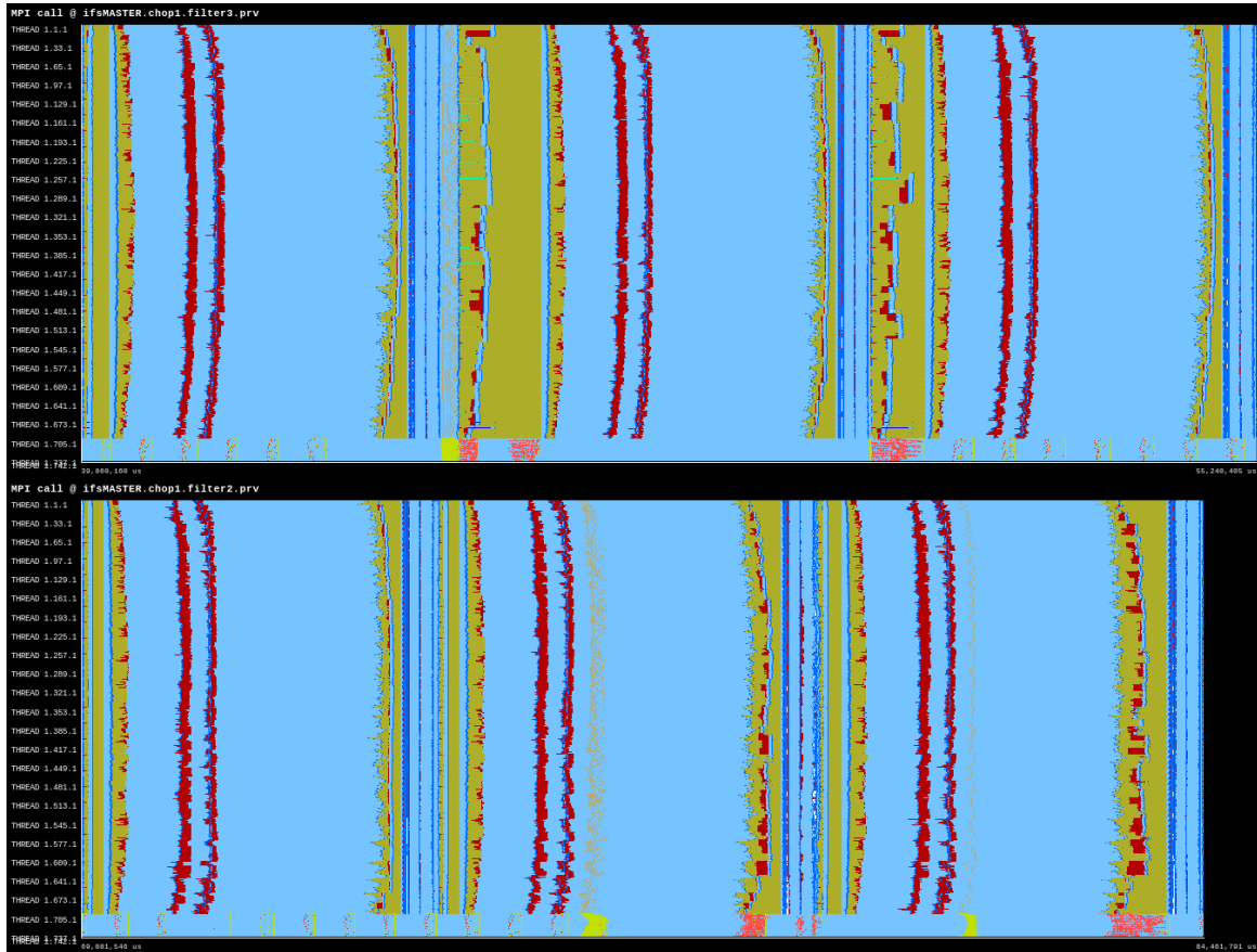
Figure 25: Trace comparison using the same elapsed time between the non-optimized overlapping (above) and the optimized overlapping (below). The three time steps of the optimized trace finish earlier than the three ones of the non-optimized trace
