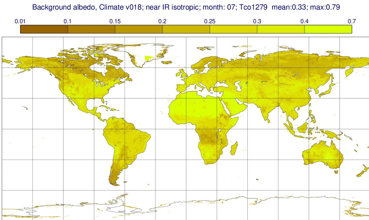
Figure 11.19 Climatological background albedo for July (near infrared, isotropic).
