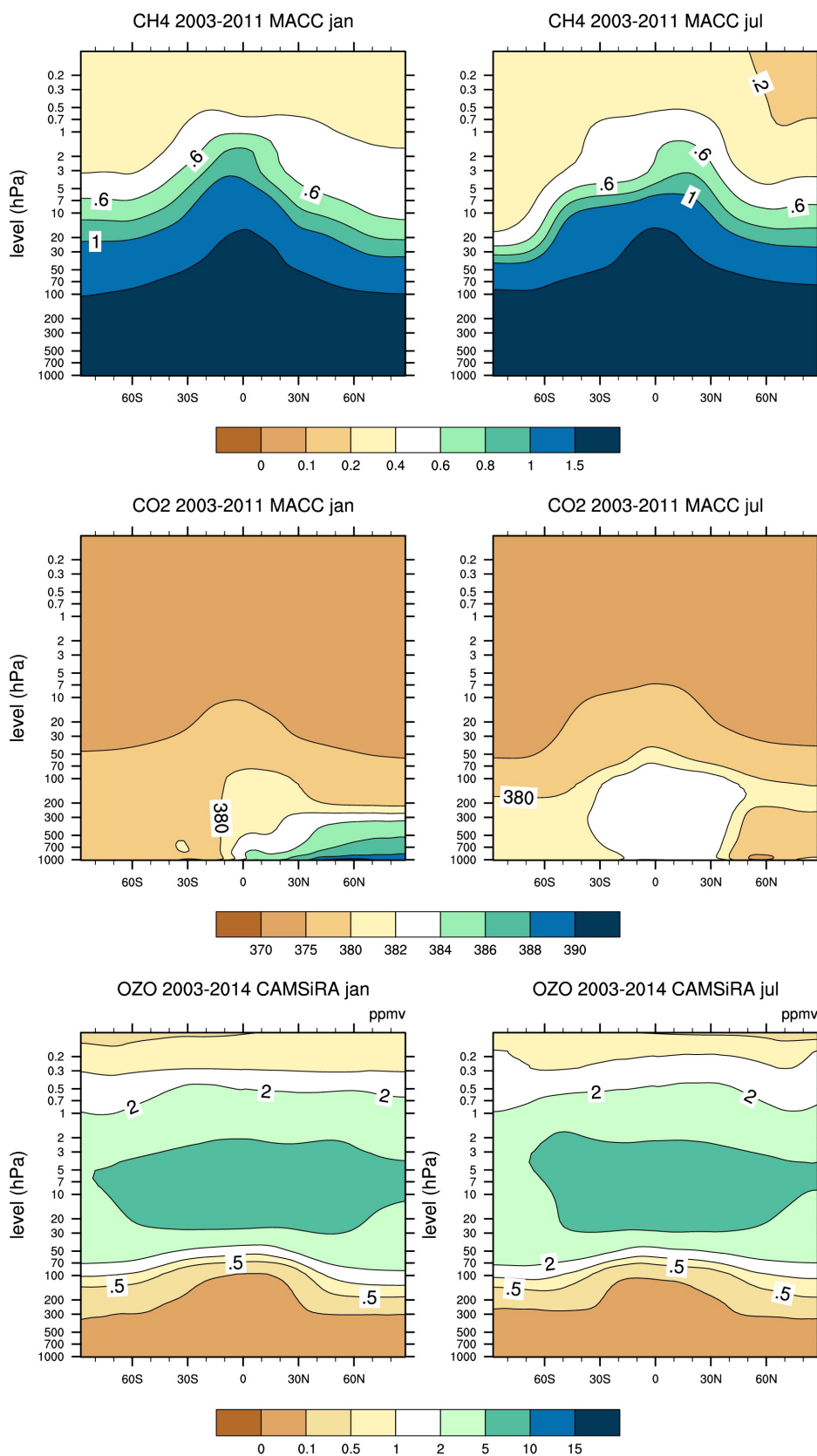
Figure 11.30 January and July monthly-mean, zonal-mean climatologies for trace gases. CO 2 , CH 4 are derived from the 2003-2011 MACC reanalysis and O 3 is derived from the 2003-2014 CAMS Interim Reanalysis. All the concentrations are in ppmv.
