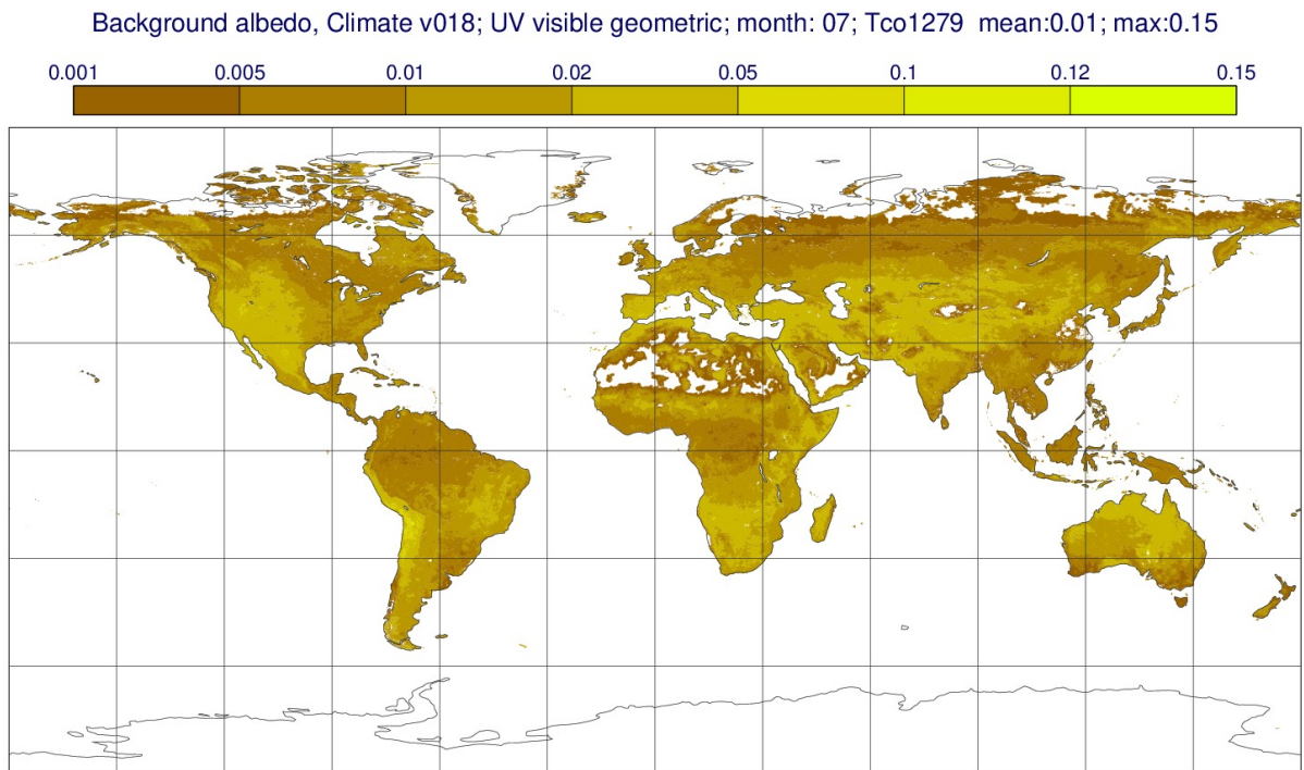
Figure 11.24 Climatological background albedo for July (UV visible, geometric).
