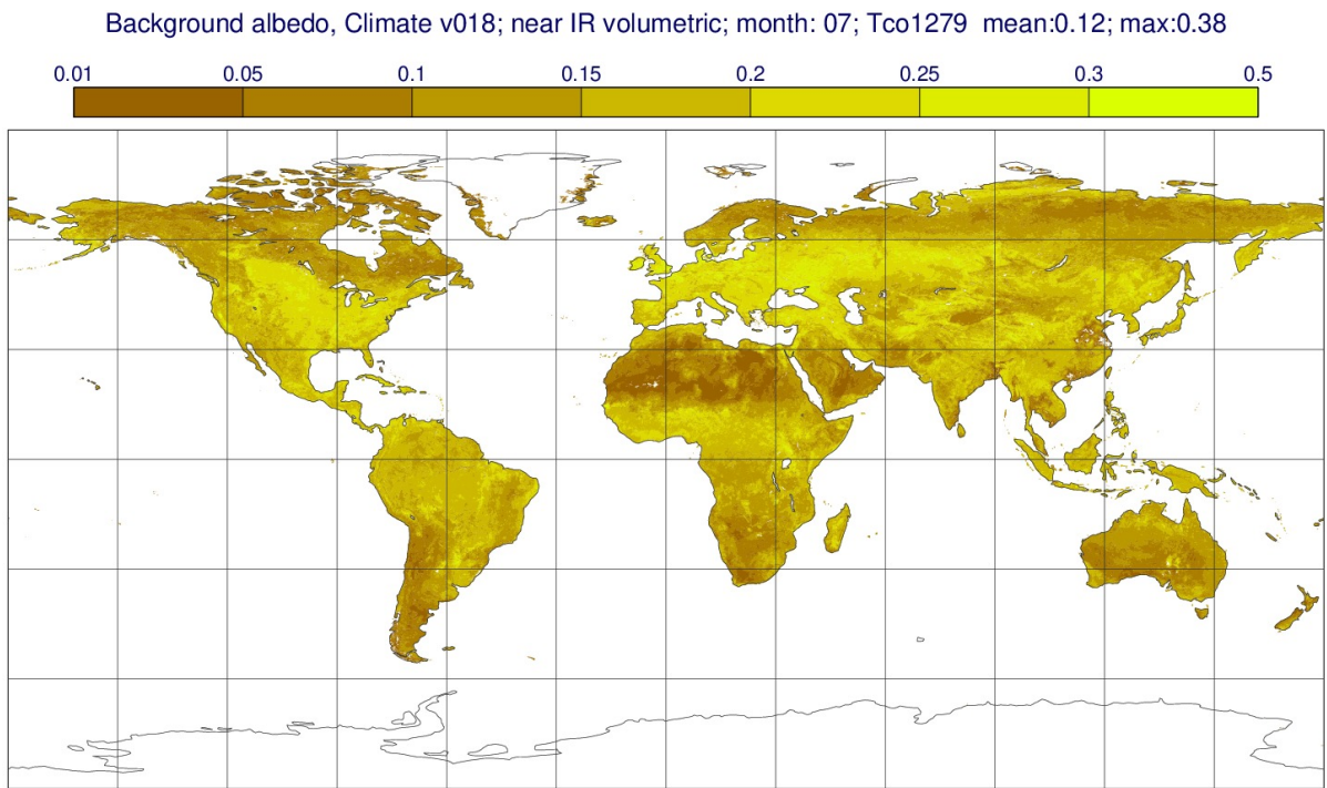
Figure 11.20 Climatological background albedo for July (near infrared, volumetric).
