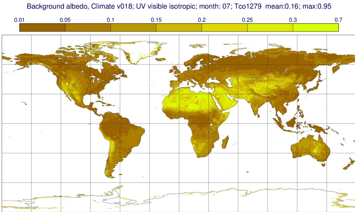
Figure 11.22 Climatological background albedo for July (UV visible, isotropic).
