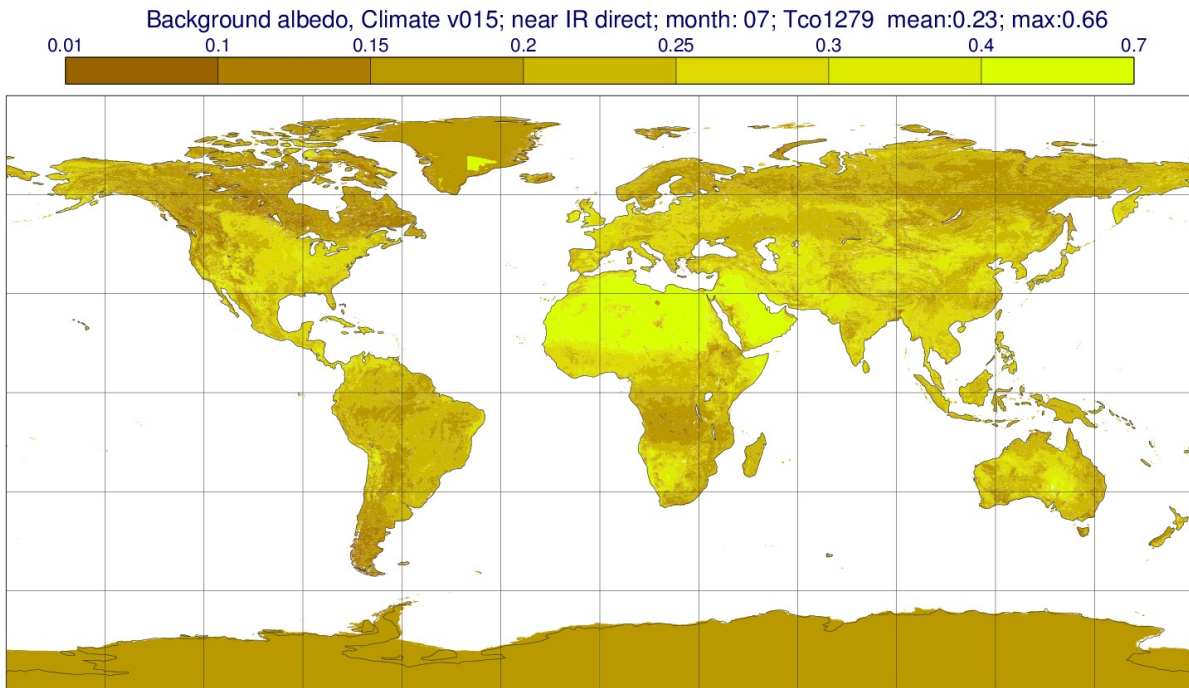
Figure 11.26 Climatological background albedo for July (near infrared, direct).
