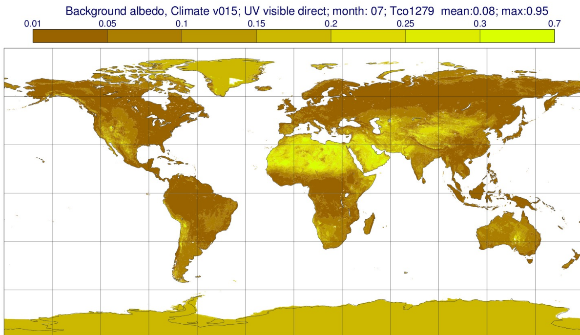
Figure 11.28 Climatological background albedo for July (UV visible, direct).
