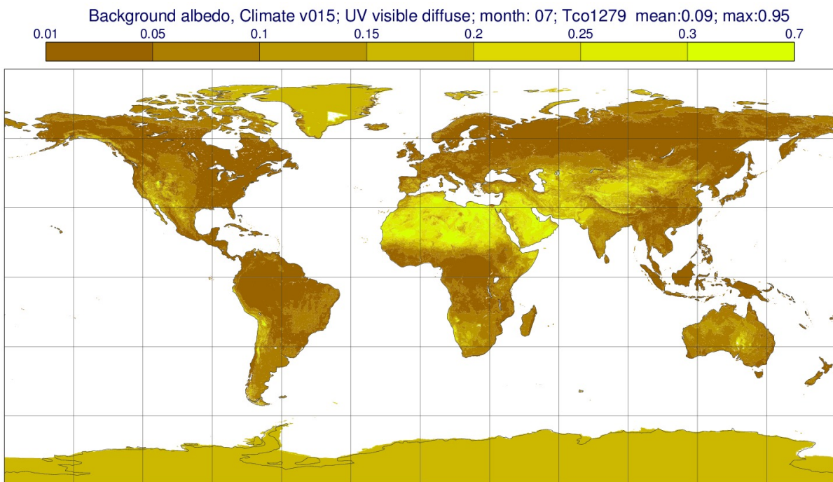
Figure 11.27 Climatological background albedo for July (UV visible, diffuse).
