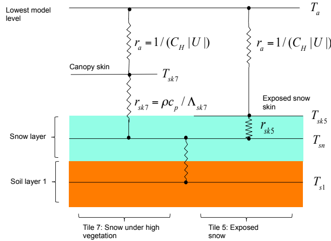
Figure 8.3 Schematic representation of the snow tiles.
