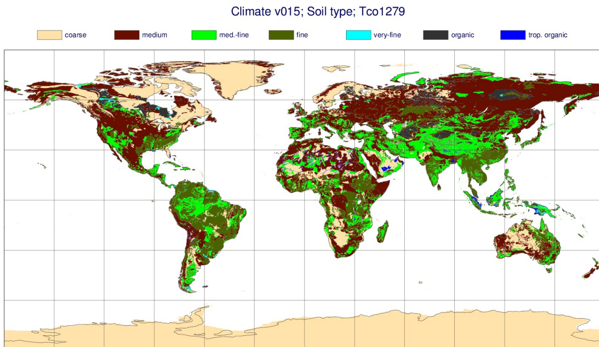
Figure 11.32 Soil type classes as used in H-TESEL.
