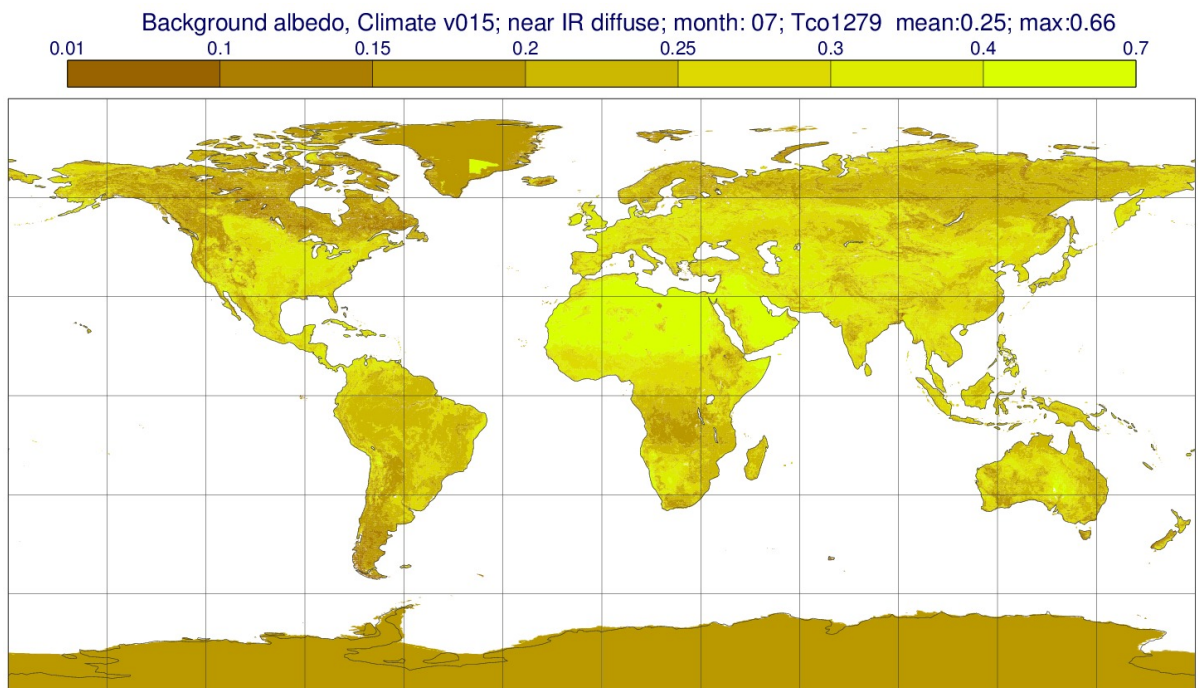
Figure 11.25 Climatological background albedo for July (near infrared, diffuse).
