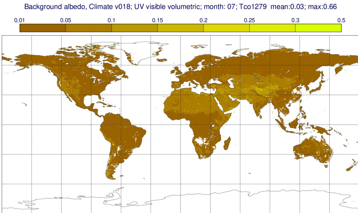
Figure 11.23 Climatological background albedo for July (UV visible, volumetric).
