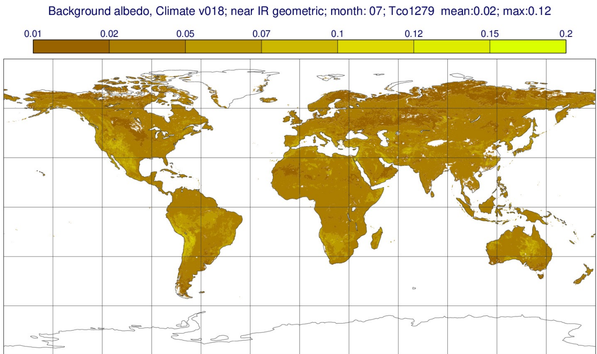
Figure 11.21 Climatological background albedo for July (near infrared, geometric).
