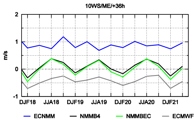
Fig.11-12 ME and MAE of ECMWF midday (36h) 10 meter wind speed forecast for seasons DJF18 to MAM21. Comparison to operational NWP models forecast.
