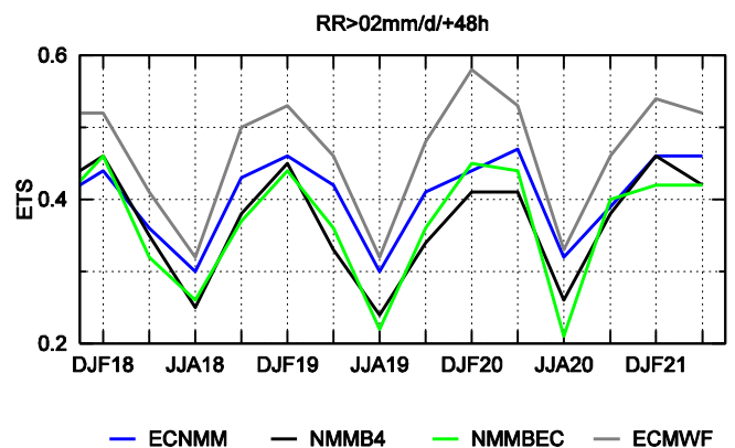
Fig.13-14 FBI and ETS of ECMWF 24h precipitation forecast (48h) for seasons DJF18 to MAM21. Threshold is 2mm/24h. Comparison to operational NWP models forecast
