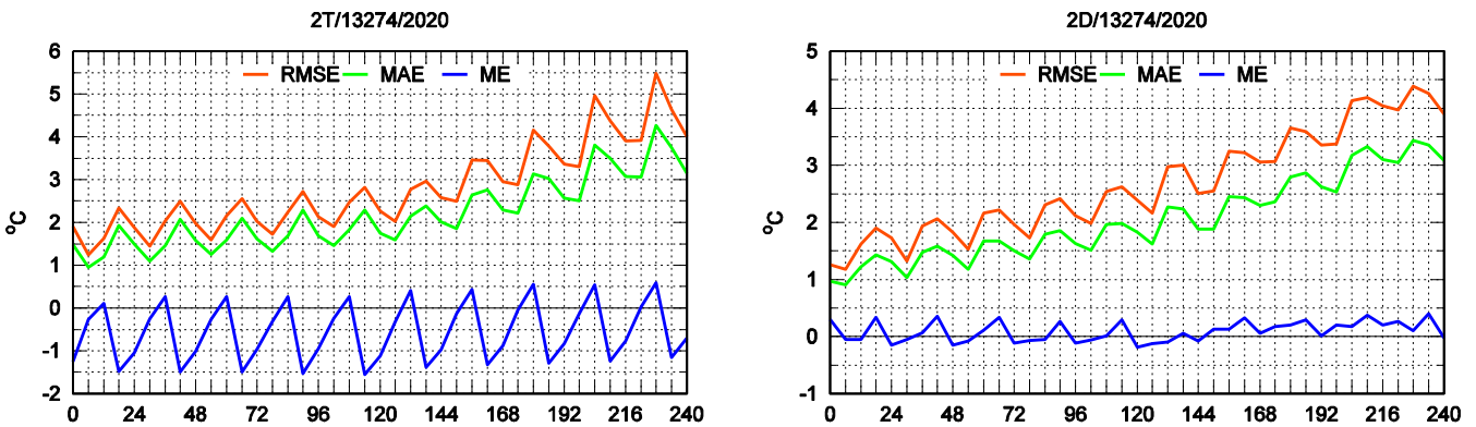
Fig.3-4 ME, MAE and RMSE of ECMWF 2 meter temperature and 2 meter dew point temperature as a function of forecast range (Beograd - Karadordev park).
