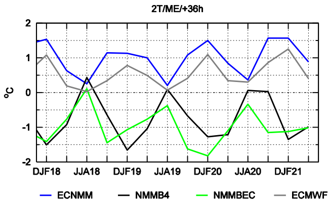
Fig.9-10 ME and MAE of ECMWF midday (36h) 2 meter temperature forecast for seasons DJF18 to MAM21. Comparison to operational NWP models forecast.
