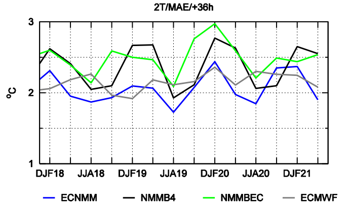
Fig.9-10 ME and MAE of ECMWF midday (36h) 2 meter temperature forecast for seasons DJF18 to MAM21. Comparison to operational NWP models forecast.
