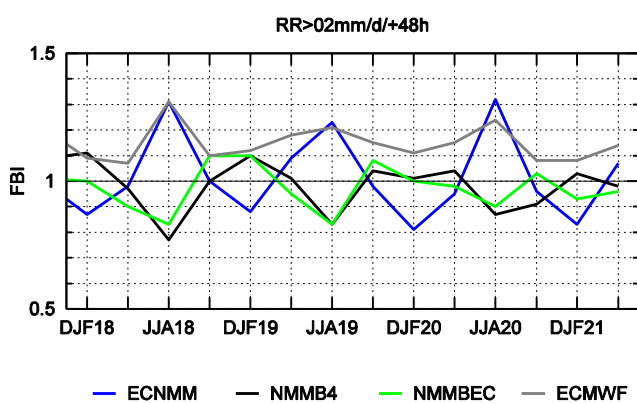
Fig.13-14 FBI and ETS of ECMWF 24h precipitation forecast (48h) for seasons DJF18 to MAM21. Threshold is 2mm/24h. Comparison to operational NWP models forecast
