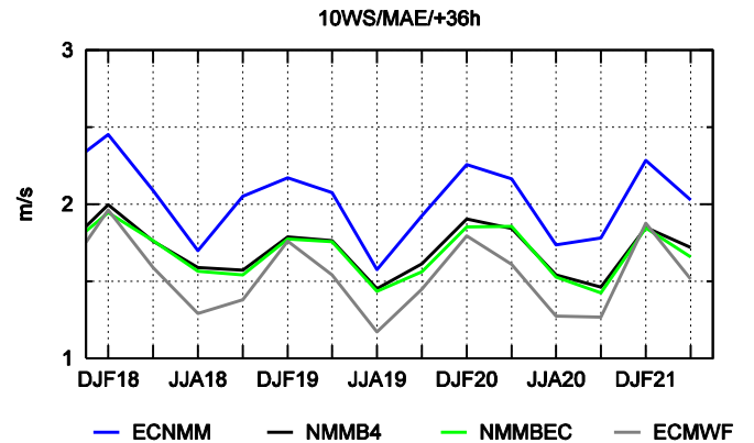
Fig.11-12 ME and MAE of ECMWF midday (36h) 10 meter wind speed forecast for seasons DJF18 to MAM21. Comparison to operational NWP models forecast.
