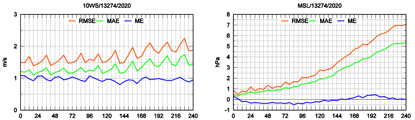
Fig.5-6 ME, MAE and RMSE of ECMWF 10 meter wind speed and mean sea level pressure forecast as a function of forecast range (Beograd - Karadordev park).
