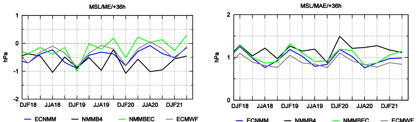
Fig.7-8 ME and MAE of ECMWF midday (36h) mean sea level pressure forecast for seasons DJF18 to MAM21. Comparison to operational NWP models forecast.
