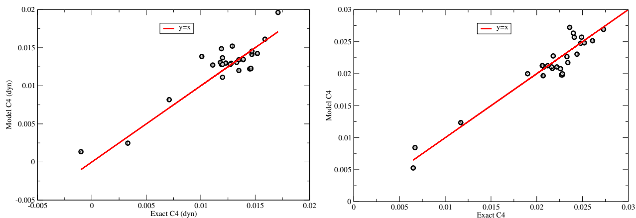
Figure 8.4 The left panel shows the comparison of parametrized dynamic kurtosis factor C_4^{dym} against exact computations using spectra from the Draupner and Andrea events, while the right panel shows the comparison for the total kurtosis factor C_4 .
