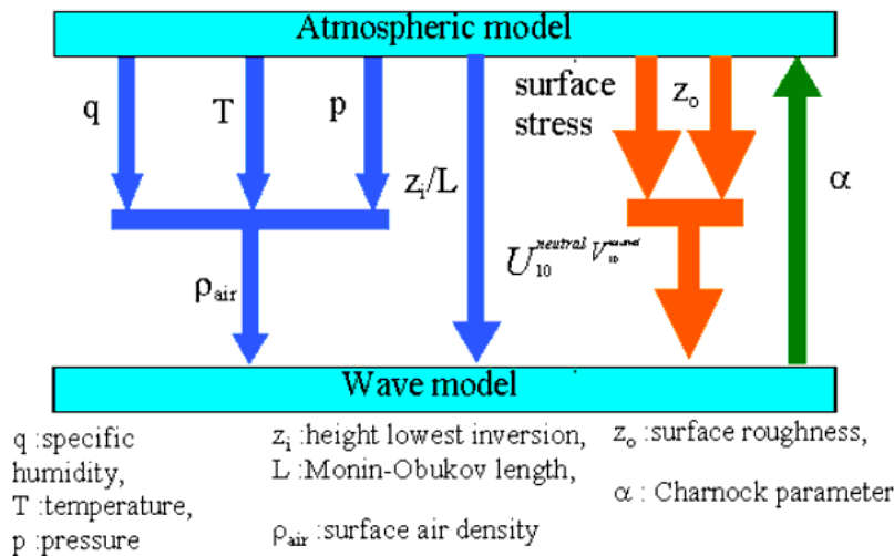
Figure 3.3 Schematic representation of the interface between the IFS and WAM.
