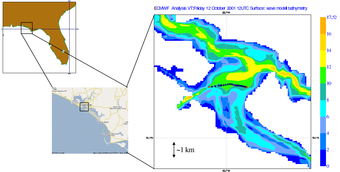
Figure 6.8 St. Andrew Bay bathymetry and trajectory of the drifting buoy where wind and waves were observed.
