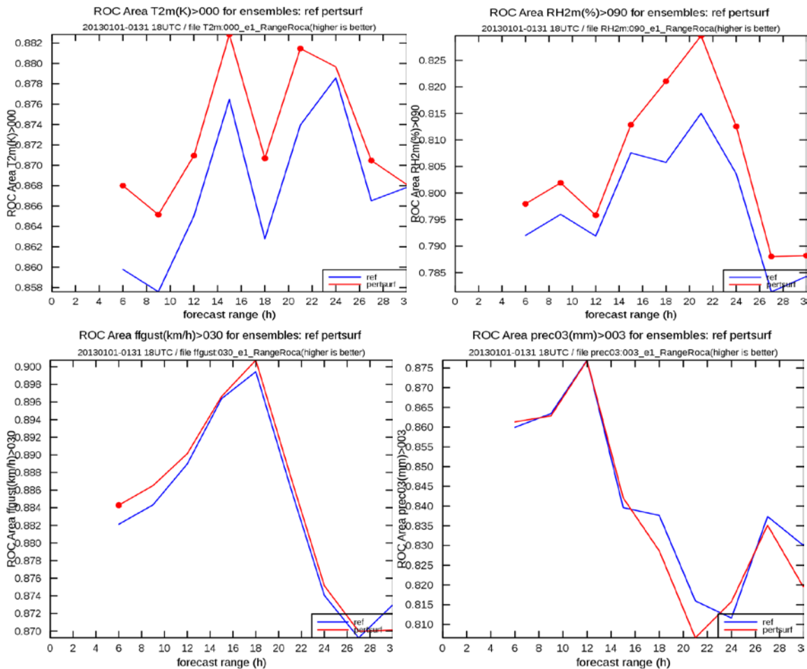
Figure: Same as on previous figure, the score now being the ROCA (Receiver Operating Characteristic Area) for the following events: T2m>0C, HU2m>90%, ff10m>30km/h, rr3h>3mm. The higher the better. These plots show that ensemble surface perturbations significantly increase the value of the ensemble for decision-making with respect to these events, for 2m temperature and humidity. The impact on windspeed and precipitation is not significant.
